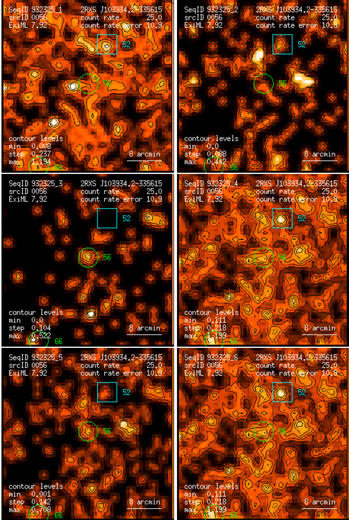
Figure 56: RASS 932325: detection 0056: band rate images, Gaussian filter: (1) PSPC channels 11 – 41, (2) 52 – 90, (3) 91 – 201, (4) 11 – 235, (5) 52 – 201, (6) 11 – 201. Broad band rates in counts/ks. Band rate contour levels in counts/ks/arcmin 2 .
