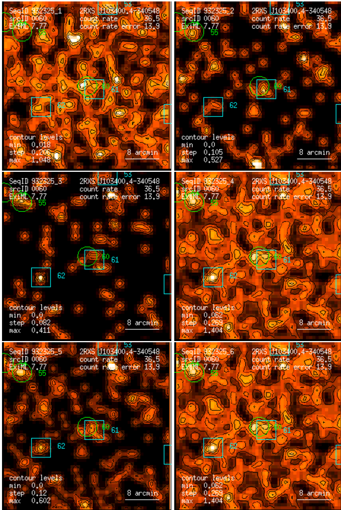
Figure 60: RASS 932325: detection 0060: band rate images, Gaussian filter: (1) PSPC channels 11 – 41, (2) 52 – 90, (3) 91 – 201, (4) 11 – 235, (5) 52 – 201, (6) 11 – 201. Broad band rates in counts/ks. Band rate contour levels in counts/ks/arcmin 2 .
