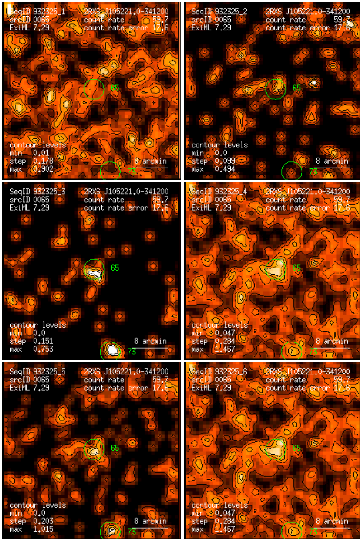
Figure 65: RASS 932325: detection 0065: band rate images, Gaussian filter: (1) PSPC channels 11 – 41, (2) 52 – 90, (3) 91 – 201, (4) 11 – 235, (5) 52 – 201, (6) 11 – 201. Broad band rates in counts/ks. Band rate contour levels in counts/ks/arcmin 2 .
