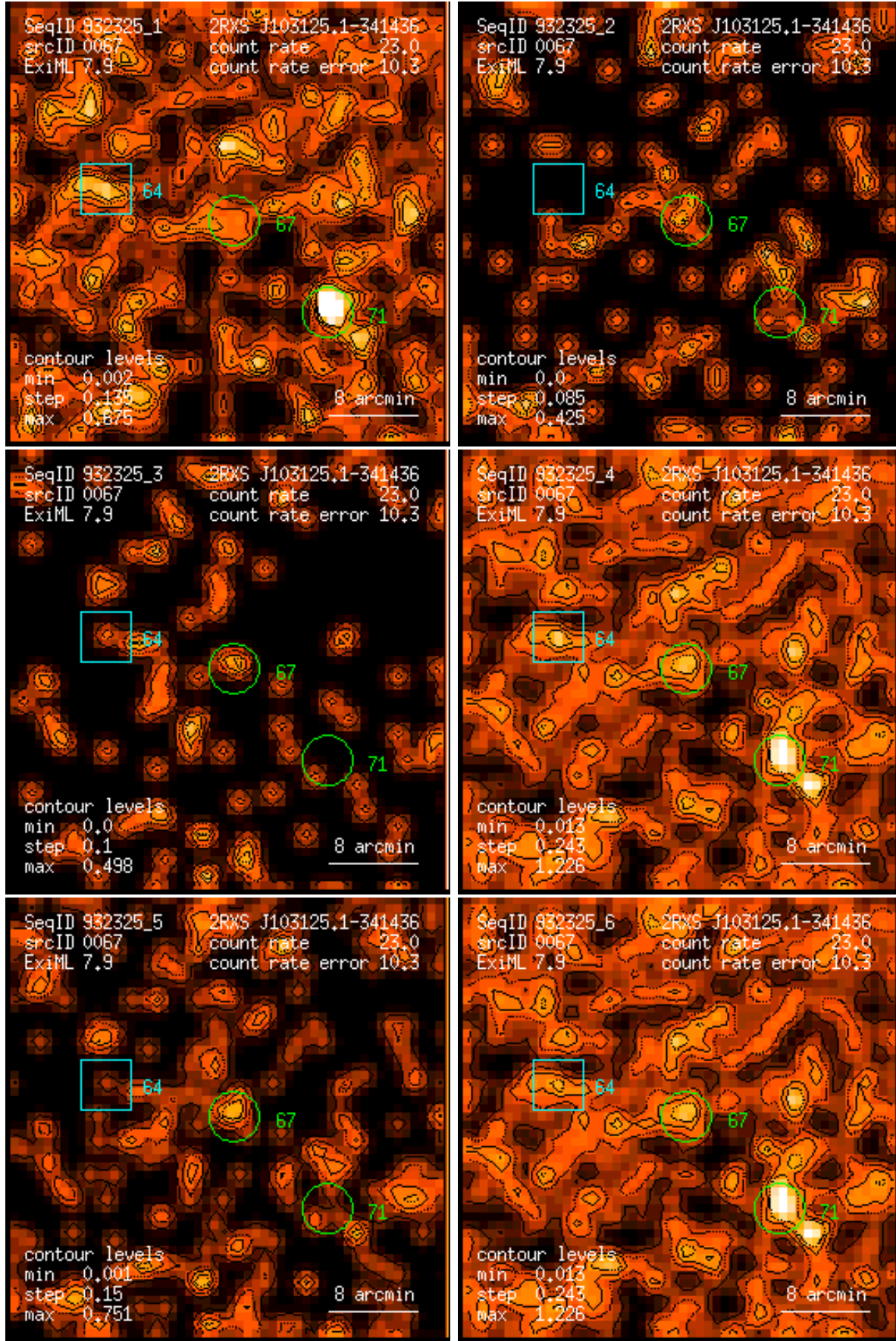
Figure 67: RASS 932325: detection 0067: band rate images, Gaussian filter: (1) PSPC channels 11 – 41, (2) 52 – 90, (3) 91 – 201, (4) 11 – 235, (5) 52 – 201, (6) 11 – 201. Broad band rates in counts/ks. Band rate contour levels in counts/ks/arcmin 2 .
