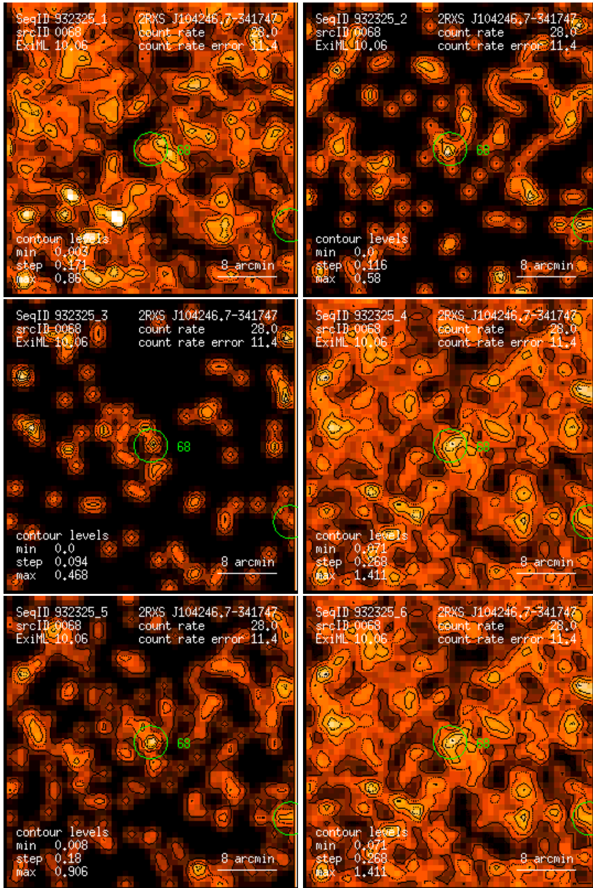
Figure 68: RASS 932325: detection 0068: band rate images, Gaussian filter: (1) PSPC channels 11 – 41, (2) 52 – 90, (3) 91 – 201, (4) 11 – 235, (5) 52 – 201, (6) 11 – 201. Broad band rates in counts/ks. Band rate contour levels in counts/ks/arcmin 2 .
