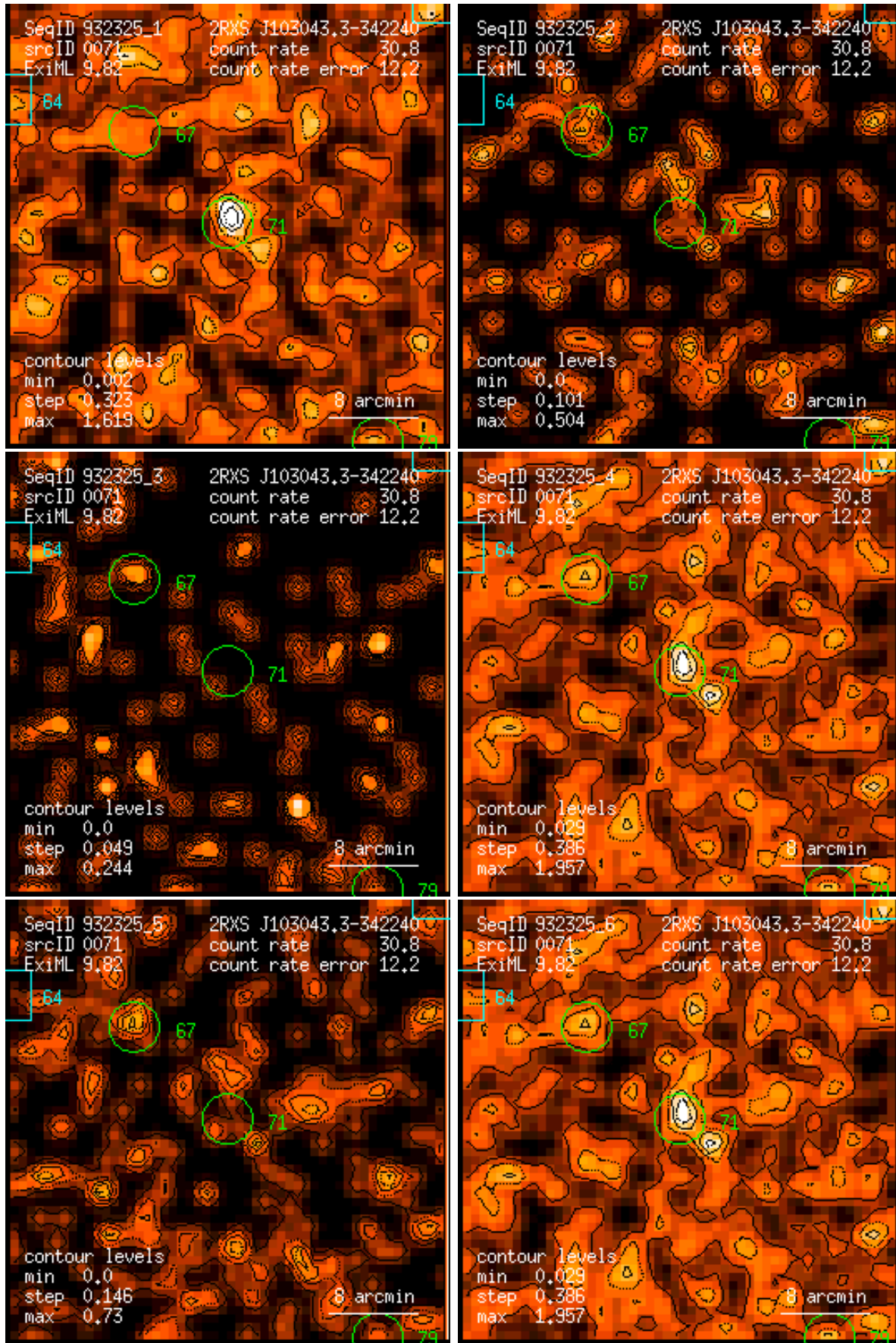
Figure 71: RASS 932325: detection 0071: band rate images, Gaussian filter: (1) PSPC channels 11 – 41, (2) 52 – 90, (3) 91 – 201, (4) 11 – 235, (5) 52 – 201, (6) 11 – 201. Broad band rates in counts/ks. Band rate contour levels in counts/ks/arcmin 2 .
