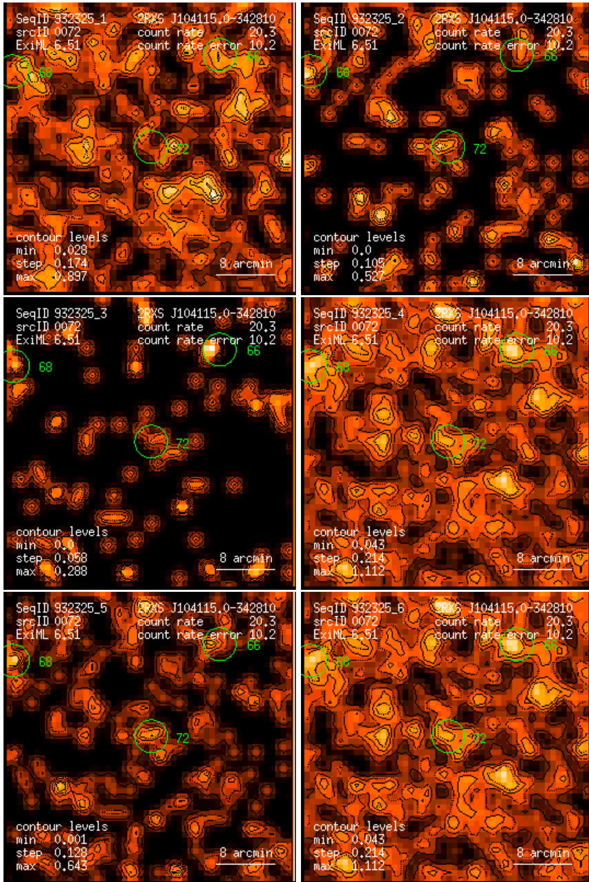
Figure 72: RASS 932325: detection 0072: band rate images, Gaussian filter: (1) PSPC channels 11 – 41, (2) 52 – 90, (3) 91 – 201, (4) 11 – 235, (5) 52 – 201, (6) 11 – 201. Broad band rates in counts/ks. Band rate contour levels in counts/ks/arcmin 2 .
