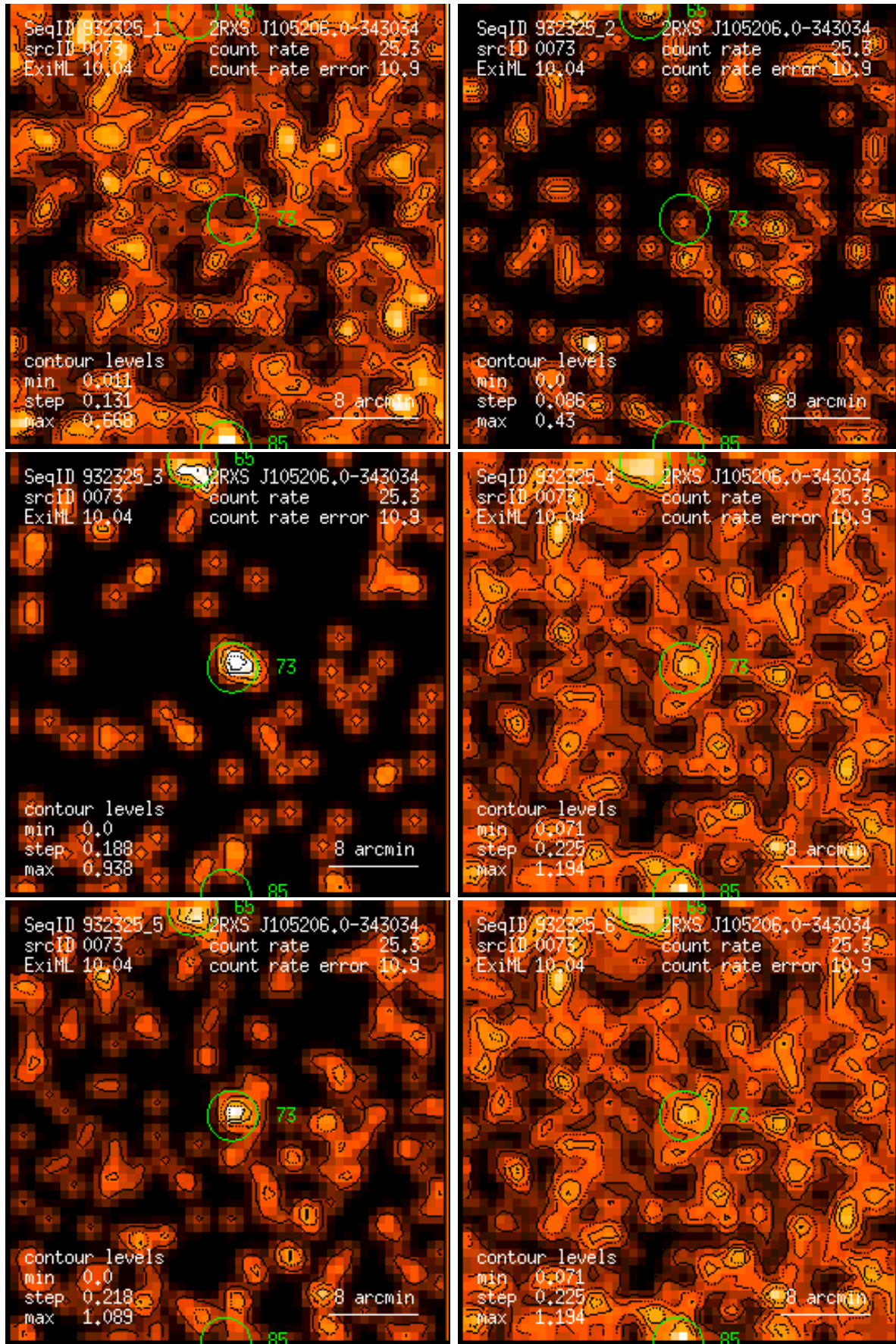
Figure 73: RASS 932325: detection 0073: band rate images, Gaussian filter: (1) PSPC channels 11 – 41, (2) 52 – 90, (3) 91 – 201, (4) 11 – 235, (5) 52 – 201, (6) 11 – 201. Broad band rates in counts/ks. Band rate contour levels in counts/ks/arcmin 2 .
