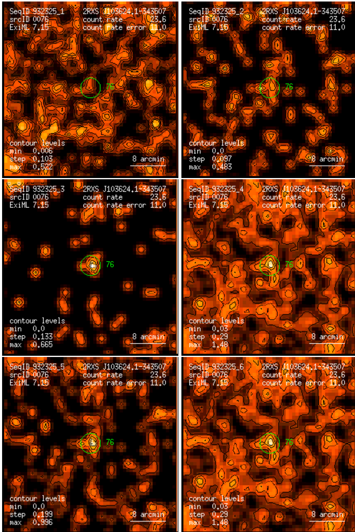
Figure 76: RASS 932325: detection 0076: band rate images, Gaussian filter: (1) PSPC channels 11 – 41, (2) 52 – 90, (3) 91 – 201, (4) 11 – 235, (5) 52 – 201, (6) 11 – 201. Broad band rates in counts/ks. Band rate contour levels in counts/ks/arcmin 2 .
