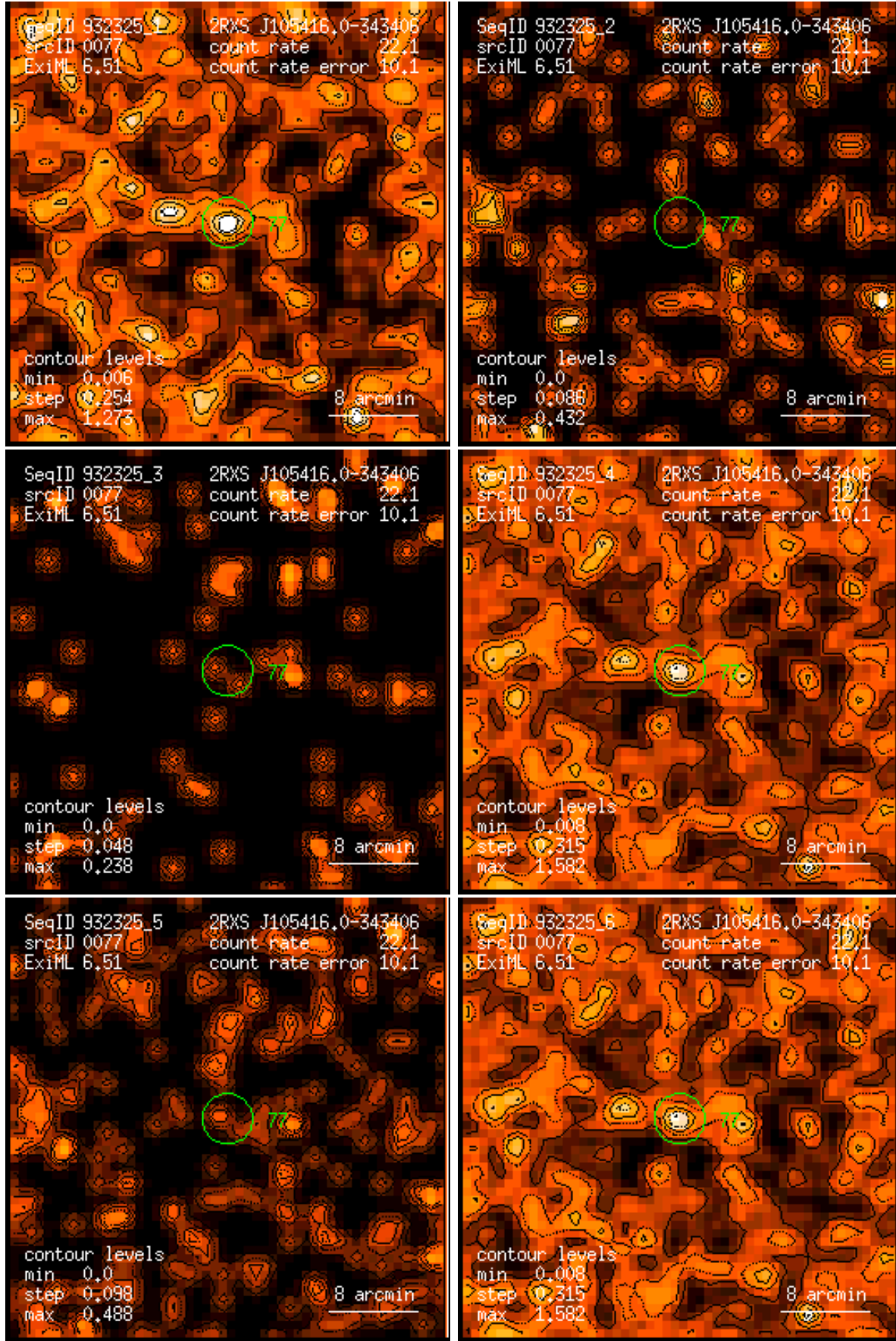
Figure 77: RASS 932325: detection 0077: band rate images, Gaussian filter: (1) PSPC channels 11 – 41, (2) 52 – 90, (3) 91 – 201, (4) 11 – 235, (5) 52 – 201, (6) 11 – 201. Broad band rates in counts/ks. Band rate contour levels in counts/ks/arcmin 2 .
