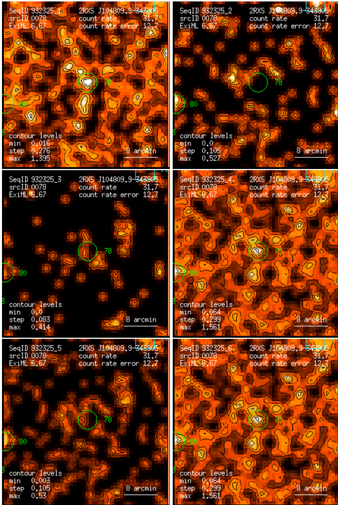
Figure 78: RASS 932325: detection 0078: band rate images, Gaussian filter: (1) PSPC channels 11 – 41, (2) 52 – 90, (3) 91 – 201, (4) 11 – 235, (5) 52 – 201, (6) 11 – 201. Broad band rates in counts/ks. Band rate contour levels in counts/ks/arcmin 2 .
