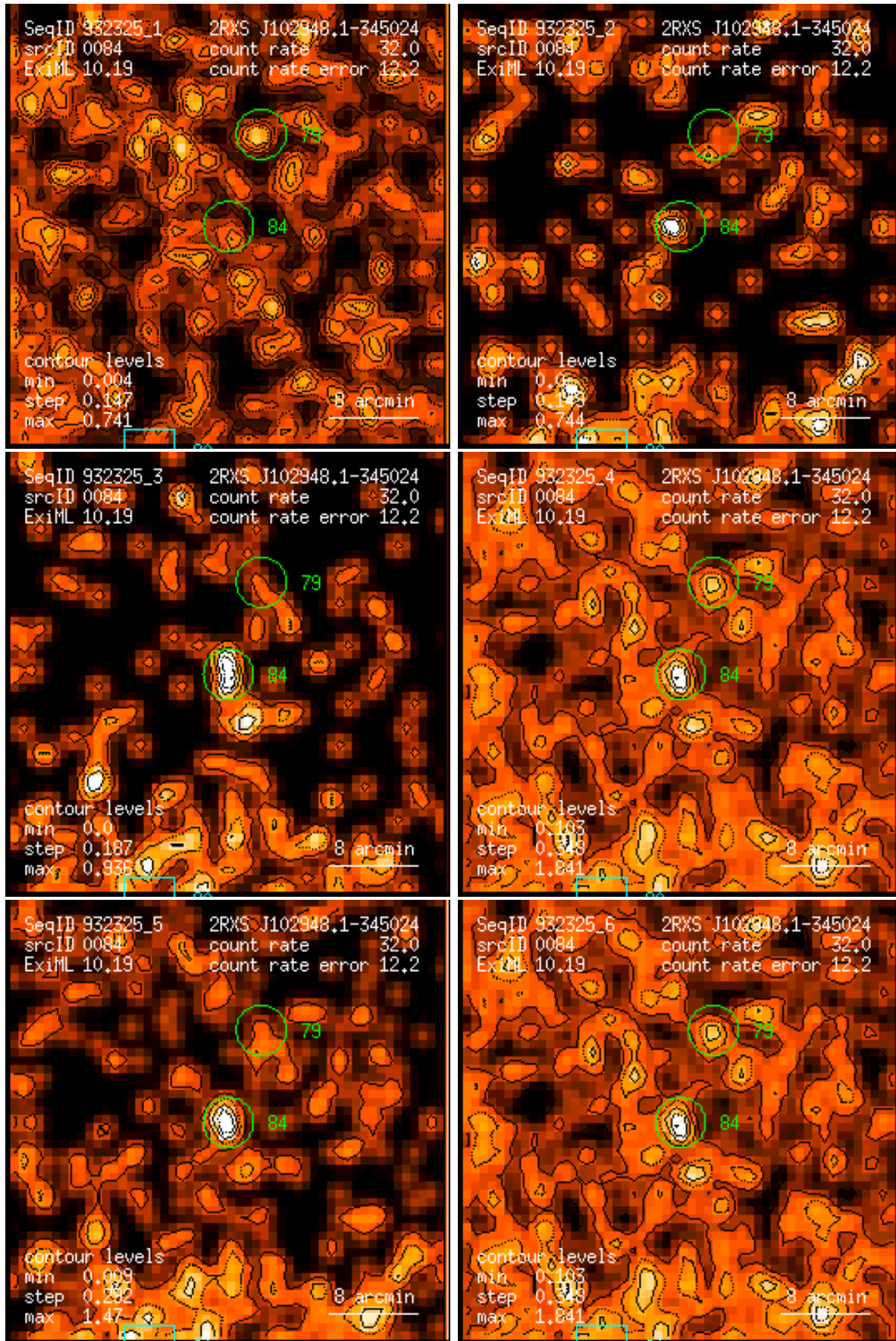
Figure 84: RASS 932325: detection 0084: band rate images, Gaussian filter: (1) PSPC channels 11 – 41, (2) 52 – 90, (3) 91 – 201, (4) 11 – 235, (5) 52 – 201, (6) 11 – 201. Broad band rates in counts/ks. Band rate contour levels in counts/ks/arcmin 2 .
