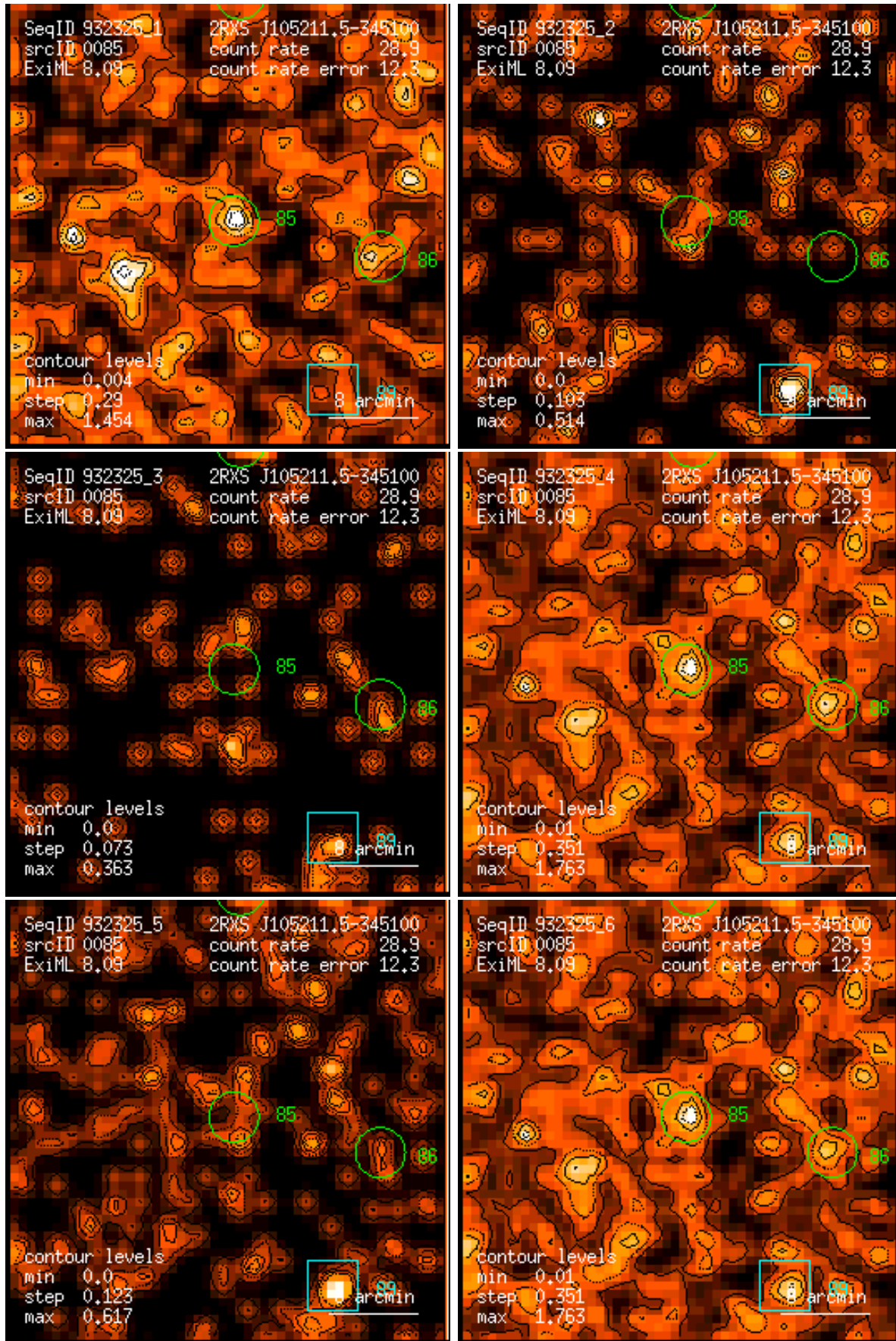
Figure 85: RASS 932325: detection 0085: band rate images, Gaussian filter: (1) PSPC channels 11 – 41, (2) 52 – 90, (3) 91 – 201, (4) 11 – 235, (5) 52 – 201, (6) 11 – 201. Broad band rates in counts/ks. Band rate contour levels in counts/ks/arcmin 2 .
