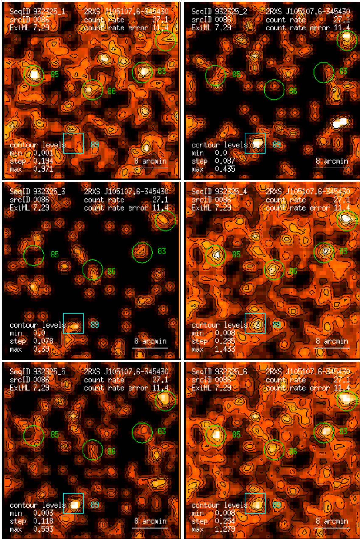
Figure 86: RASS 932325: detection 0086: band rate images, Gaussian filter: (1) PSPC channels 11 – 41, (2) 52 – 90, (3) 91 – 201, (4) 11 – 235, (5) 52 – 201, (6) 11 – 201. Broad band rates in counts/ks. Band rate contour levels in counts/ks/arcmin 2 .
