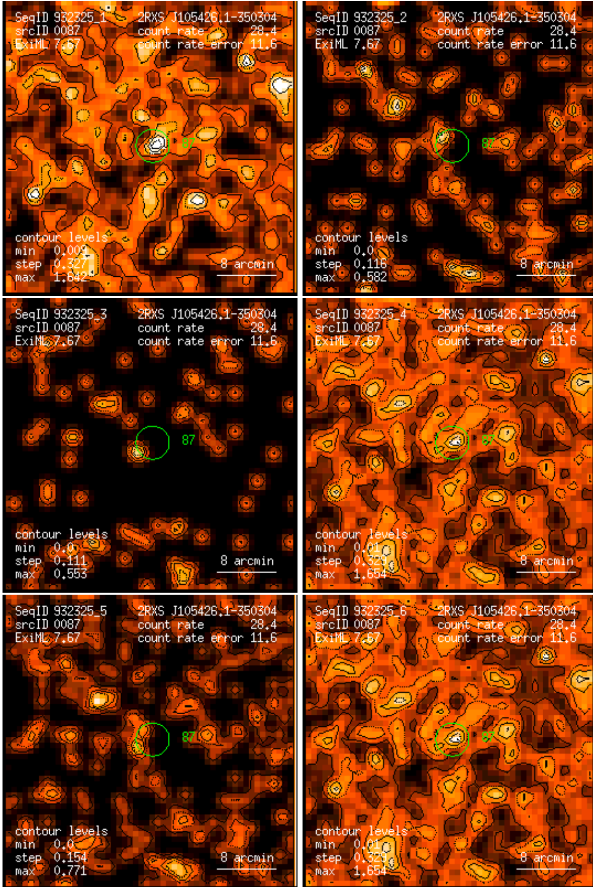
Figure 87: RASS 932325: detection 0087: band rate images, Gaussian filter: (1) PSPC channels 11 – 41, (2) 52 – 90, (3) 91 – 201, (4) 11 – 235, (5) 52 – 201, (6) 11 – 201. Broad band rates in counts/ks. Band rate contour levels in counts/ks/arcmin 2 .
