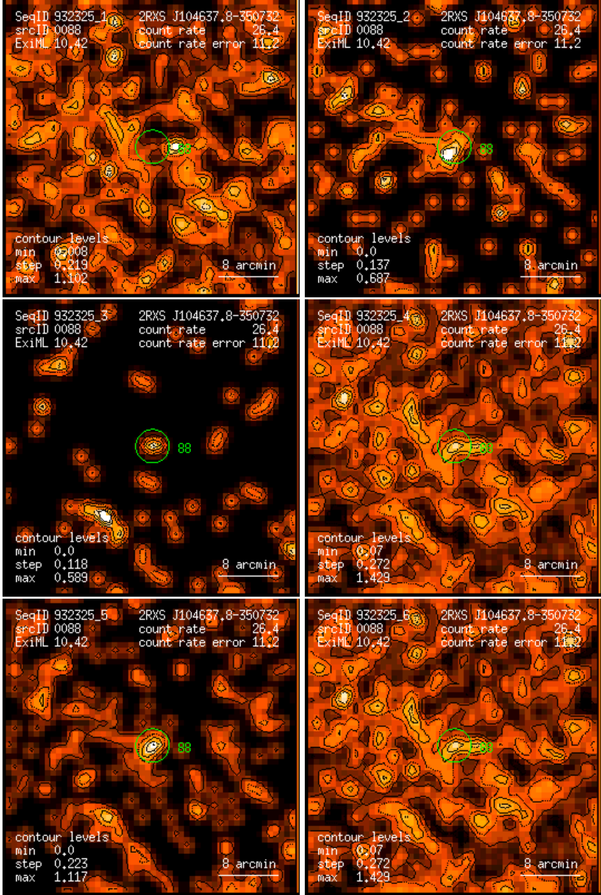
Figure 88: RASS 932325: detection 0088: band rate images, Gaussian filter: (1) PSPC channels 11 – 41, (2) 52 – 90, (3) 91 – 201, (4) 11 – 235, (5) 52 – 201, (6) 11 – 201. Broad band rates in counts/ks. Band rate contour levels in counts/ks/arcmin 2 .
