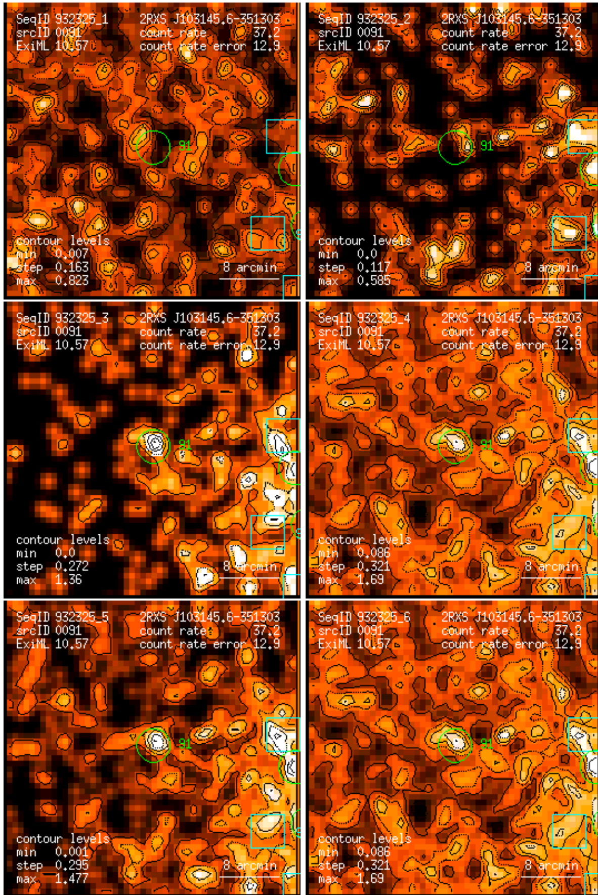
Figure 91: RASS 932325: detection 0091: band rate images, Gaussian filter: (1) PSPC channels 11 – 41, (2) 52 – 90, (3) 91 – 201, (4) 11 – 235, (5) 52 – 201, (6) 11 – 201. Broad band rates in counts/ks. Band rate contour levels in counts/ks/arcmin 2 .
