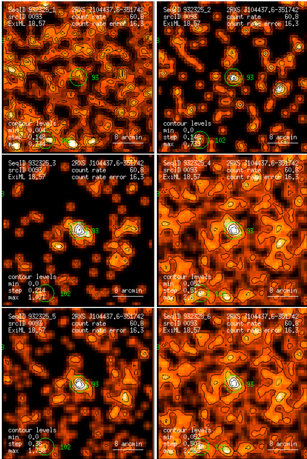
Figure 93: RASS 932325: detection 0093: band rate images, Gaussian filter: (1) PSPC channels 11 – 41, (2) 52 – 90, (3) 91 – 201, (4) 11 – 235, (5) 52 – 201, (6) 11 – 201. Broad band rates in counts/ks. Band rate contour levels in counts/ks/arcmin 2 .
