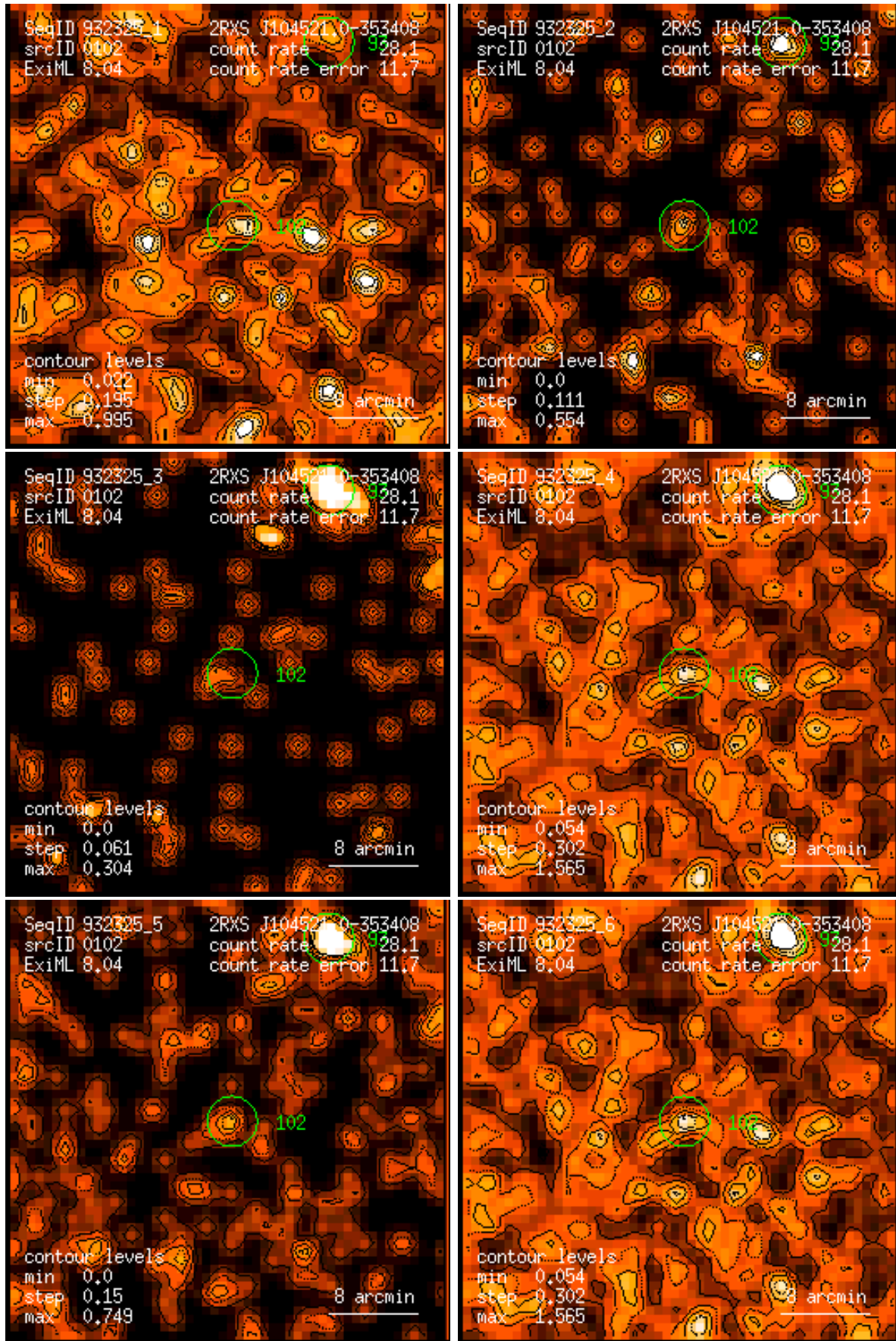
Figure 102: RASS 932325: detection 0102: band rate images, Gaussian filter: (1) PSPC channels 11 – 41, (2) 52 – 90, (3) 91 – 201, (4) 11 – 235, (5) 52 – 201, (6) 11 – 201. Broad band rates in counts/ks. Band rate contour levels in counts/ks/arcmin 2 .
