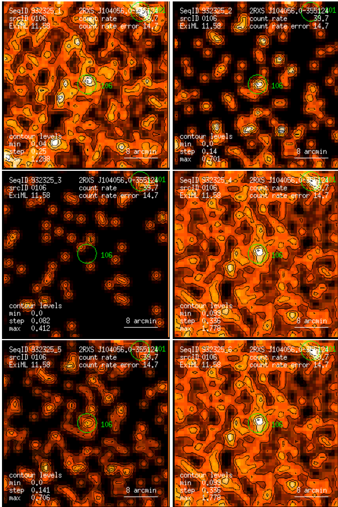
Figure 106: RASS 932325: detection 0106: band rate images, Gaussian filter: (1) PSPC channels 11 – 41, (2) 52 – 90, (3) 91 – 201, (4) 11 – 235, (5) 52 – 201, (6) 11 – 201. Broad band rates in counts/ks. Band rate contour levels in counts/ks/arcmin 2 .
