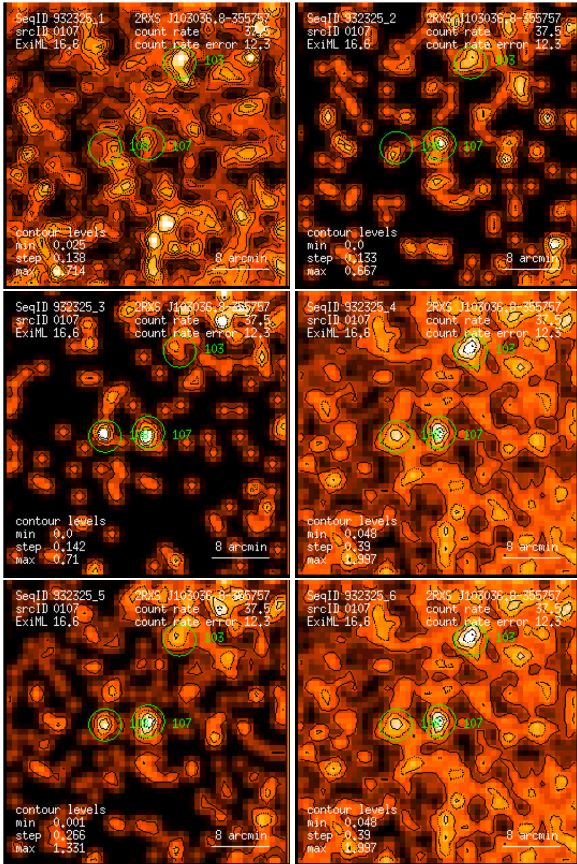
Figure 107: RASS 932325: detection 0107: band rate images, Gaussian filter: (1) PSPC channels 11 – 41, (2) 52 – 90, (3) 91 – 201, (4) 11 – 235, (5) 52 – 201, (6) 11 – 201. Broad band rates in counts/ks. Band rate contour levels in counts/ks/arcmin 2 .
