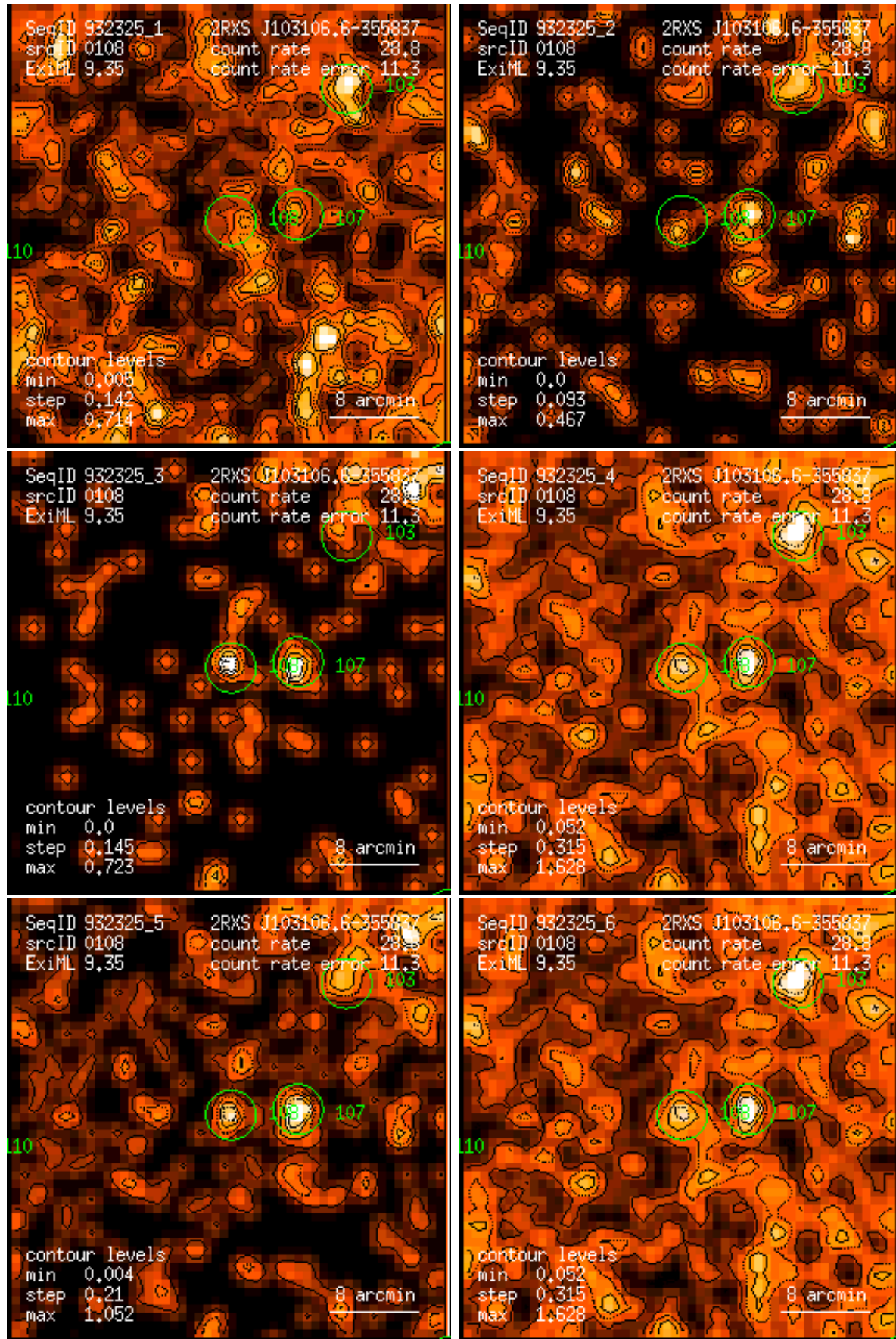
Figure 108: RASS 932325: detection 0108: band rate images, Gaussian filter: (1) PSPC channels 11 – 41, (2) 52 – 90, (3) 91 – 201, (4) 11 – 235, (5) 52 – 201, (6) 11 – 201. Broad band rates in counts/ks. Band rate contour levels in counts/ks/arcmin 2 .
