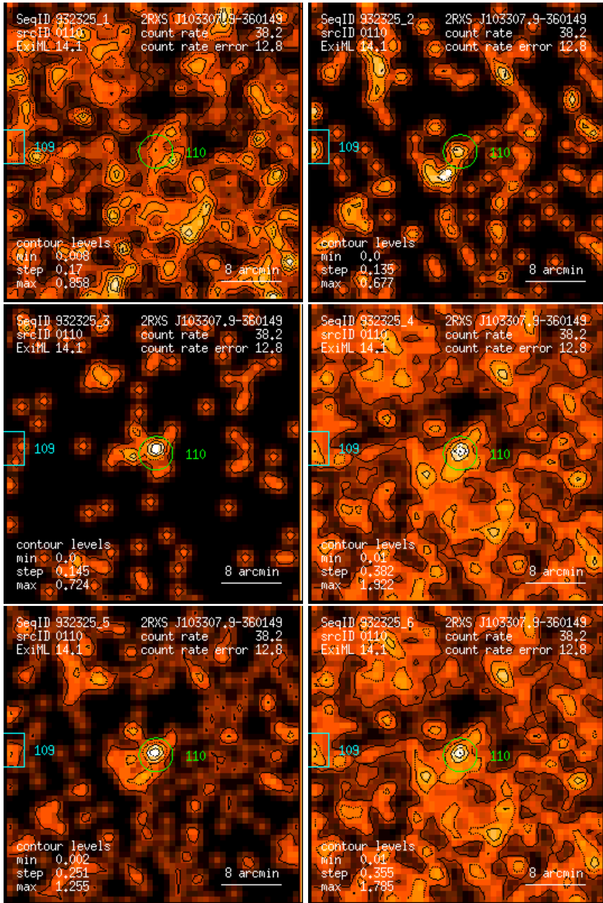
Figure 110: RASS 932325: detection 0110: band rate images, Gaussian filter: (1) PSPC channels 11 – 41, (2) 52 – 90, (3) 91 – 201, (4) 11 – 235, (5) 52 – 201, (6) 11 – 201. Broad band rates in counts/ks. Band rate contour levels in counts/ks/arcmin 2 .
