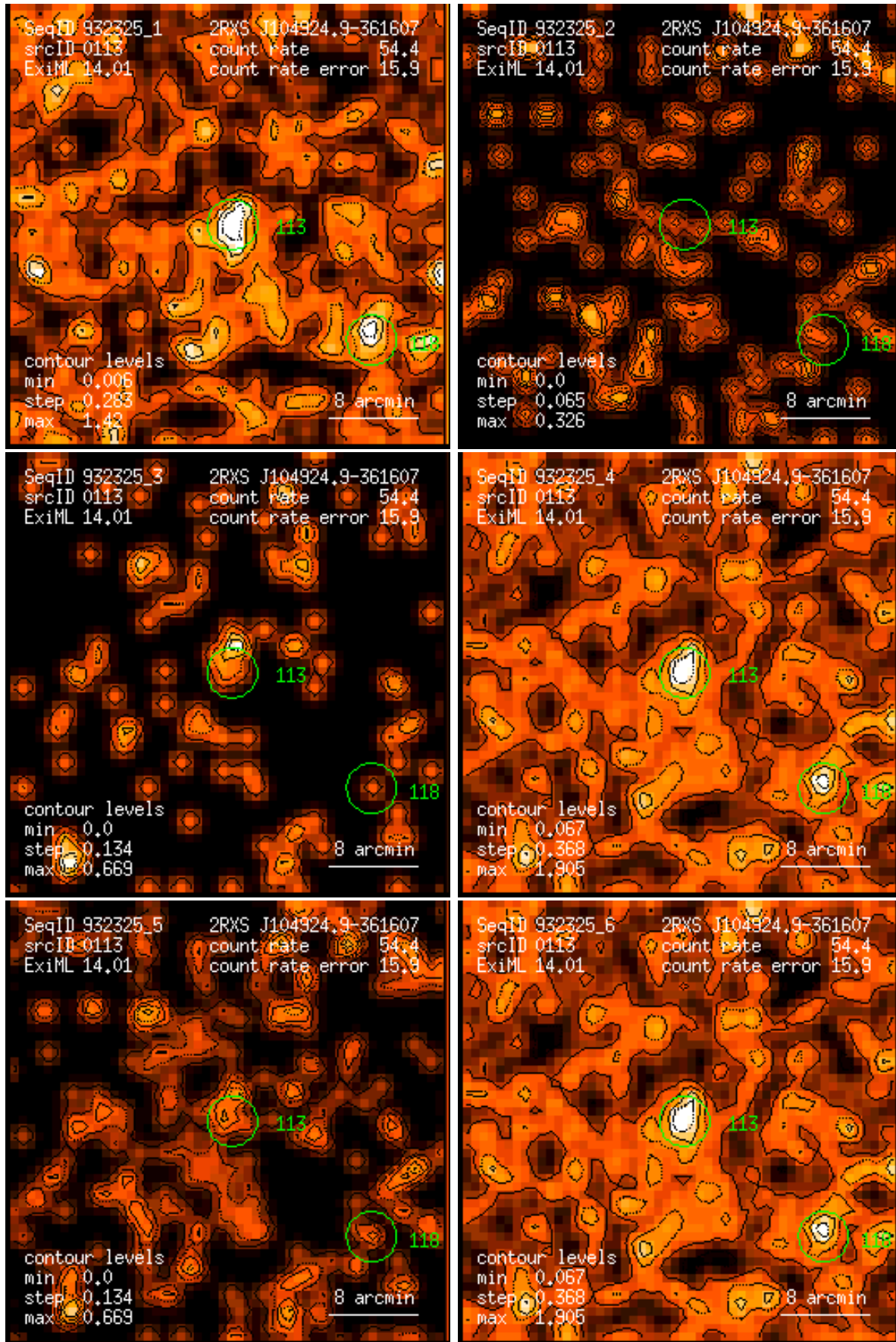
Figure 113: RASS 932325: detection 0113: band rate images, Gaussian filter: (1) PSPC channels 11 – 41, (2) 52 – 90, (3) 91 – 201, (4) 11 – 235, (5) 52 – 201, (6) 11 – 201. Broad band rates in counts/ks. Band rate contour levels in counts/ks/arcmin 2 .
