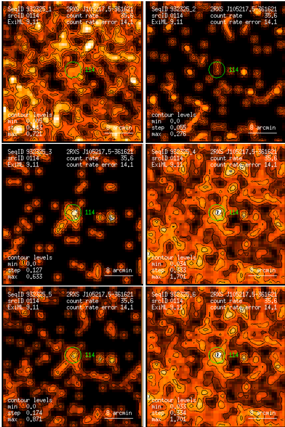
Figure 114: RASS 932325: detection 0114: band rate images, Gaussian filter: (1) PSPC channels 11 – 41, (2) 52 – 90, (3) 91 – 201, (4) 11 – 235, (5) 52 – 201, (6) 11 – 201. Broad band rates in counts/ks. Band rate contour levels in counts/ks/arcmin 2 .
