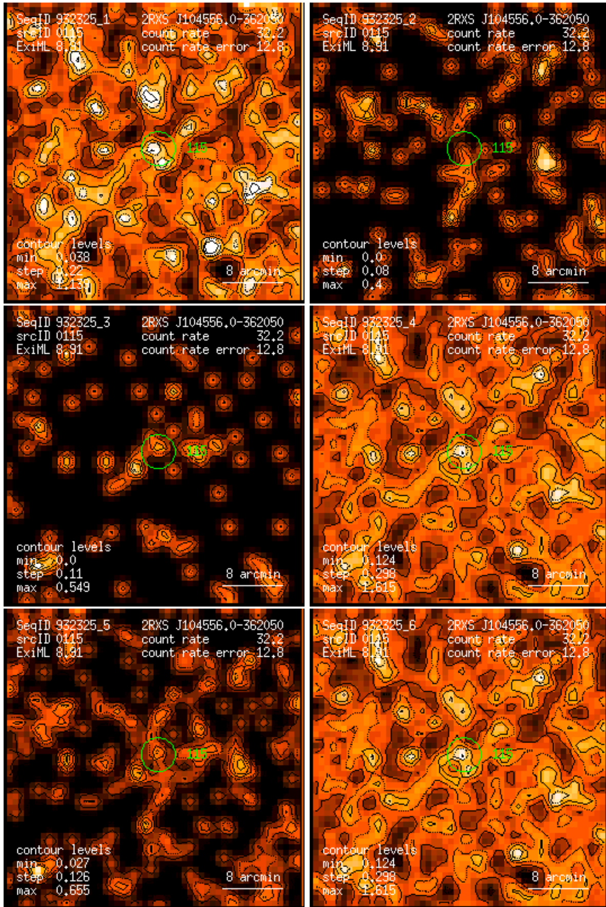
Figure 115: RASS 932325: detection 0115: band rate images, Gaussian filter: (1) PSPC channels 11 – 41, (2) 52 – 90, (3) 91 – 201, (4) 11 – 235, (5) 52 – 201, (6) 11 – 201. Broad band rates in counts/ks. Band rate contour levels in counts/ks/arcmin 2 .
