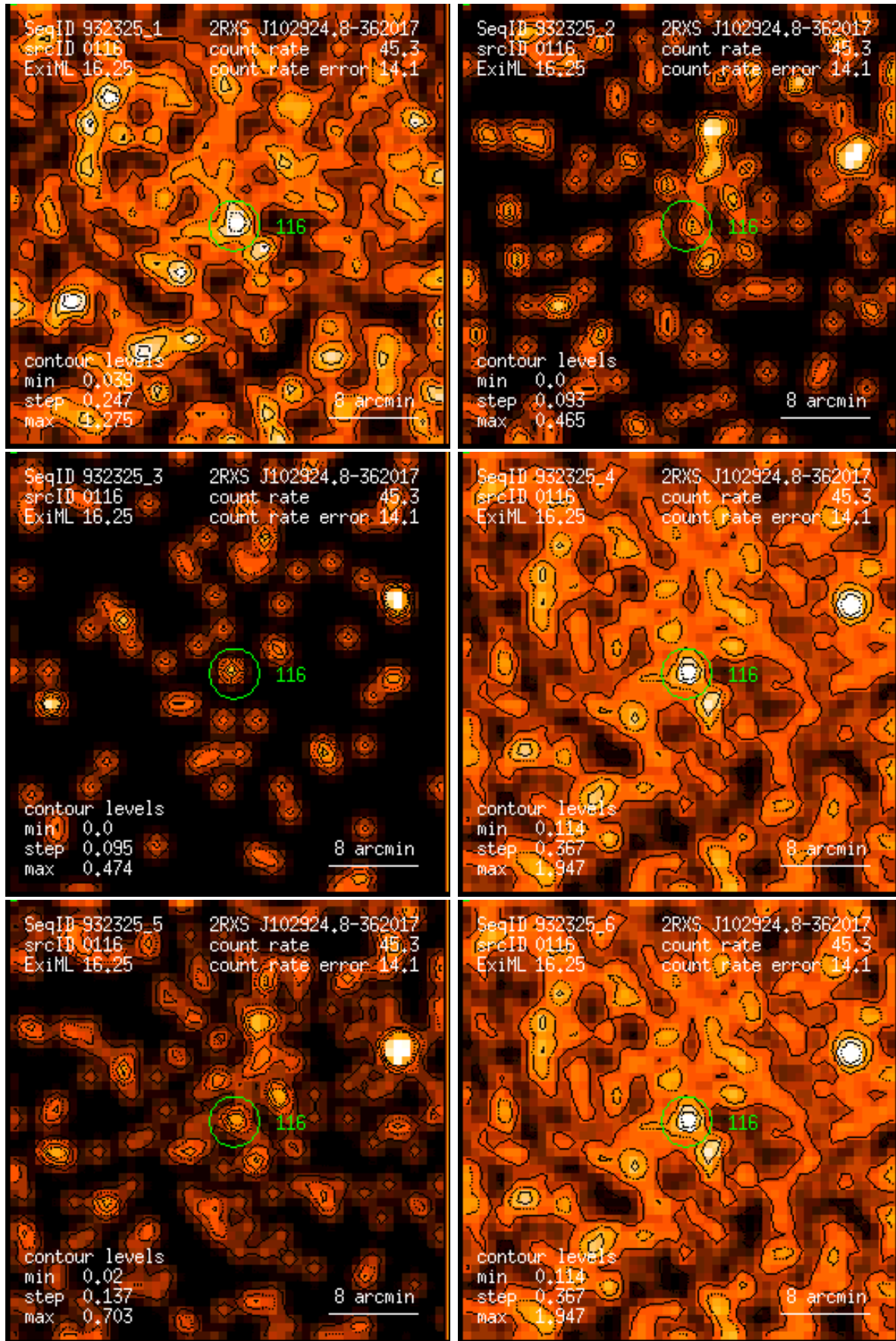
Figure 116: RASS 932325: detection 0116: band rate images, Gaussian filter: (1) PSPC channels 11 – 41, (2) 52 – 90, (3) 91 – 201, (4) 11 – 235, (5) 52 – 201, (6) 11 – 201. Broad band rates in counts/ks. Band rate contour levels in counts/ks/arcmin 2 .
