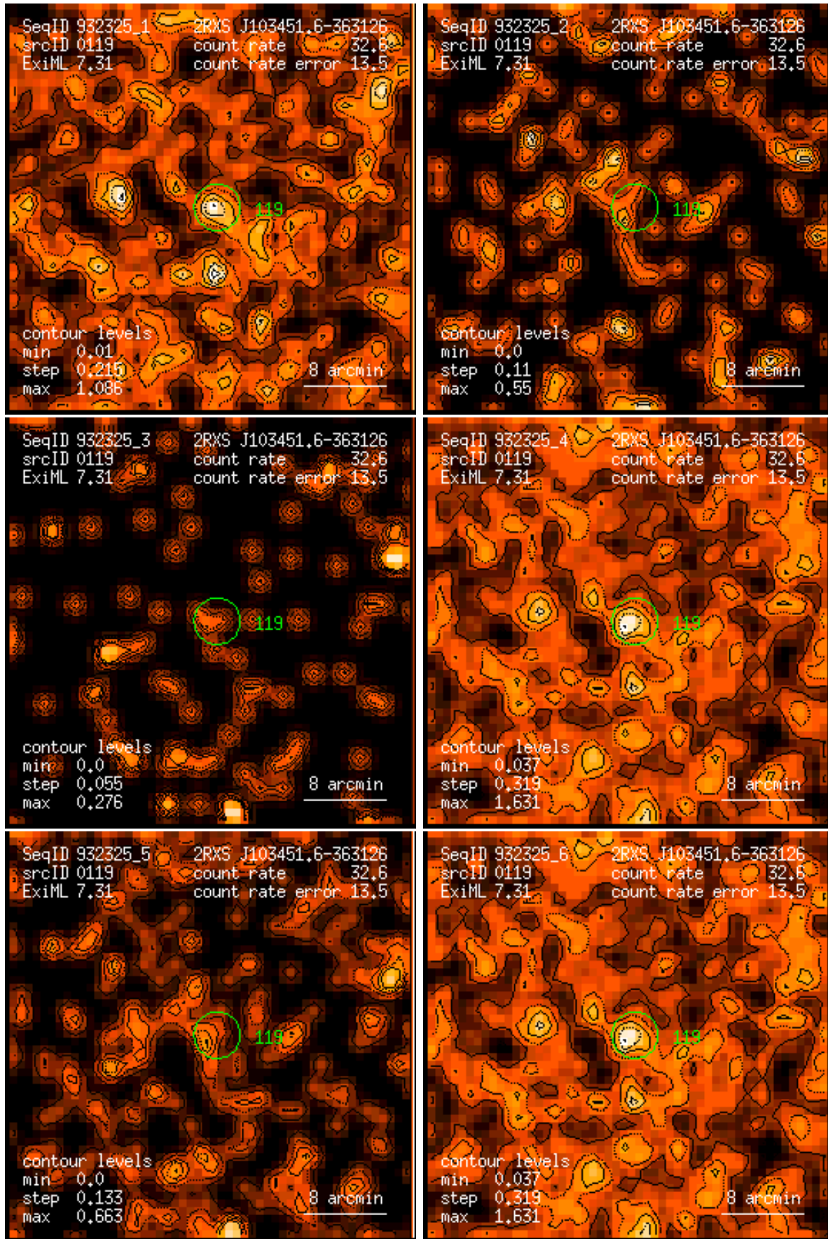
Figure 119: RASS 932325: detection 0119: band rate images, Gaussian filter: (1) PSPC channels 11 – 41, (2) 52 – 90, (3) 91 – 201, (4) 11 – 235, (5) 52 – 201, (6) 11 – 201. Broad band rates in counts/ks. Band rate contour levels in counts/ks/arcmin 2 .
