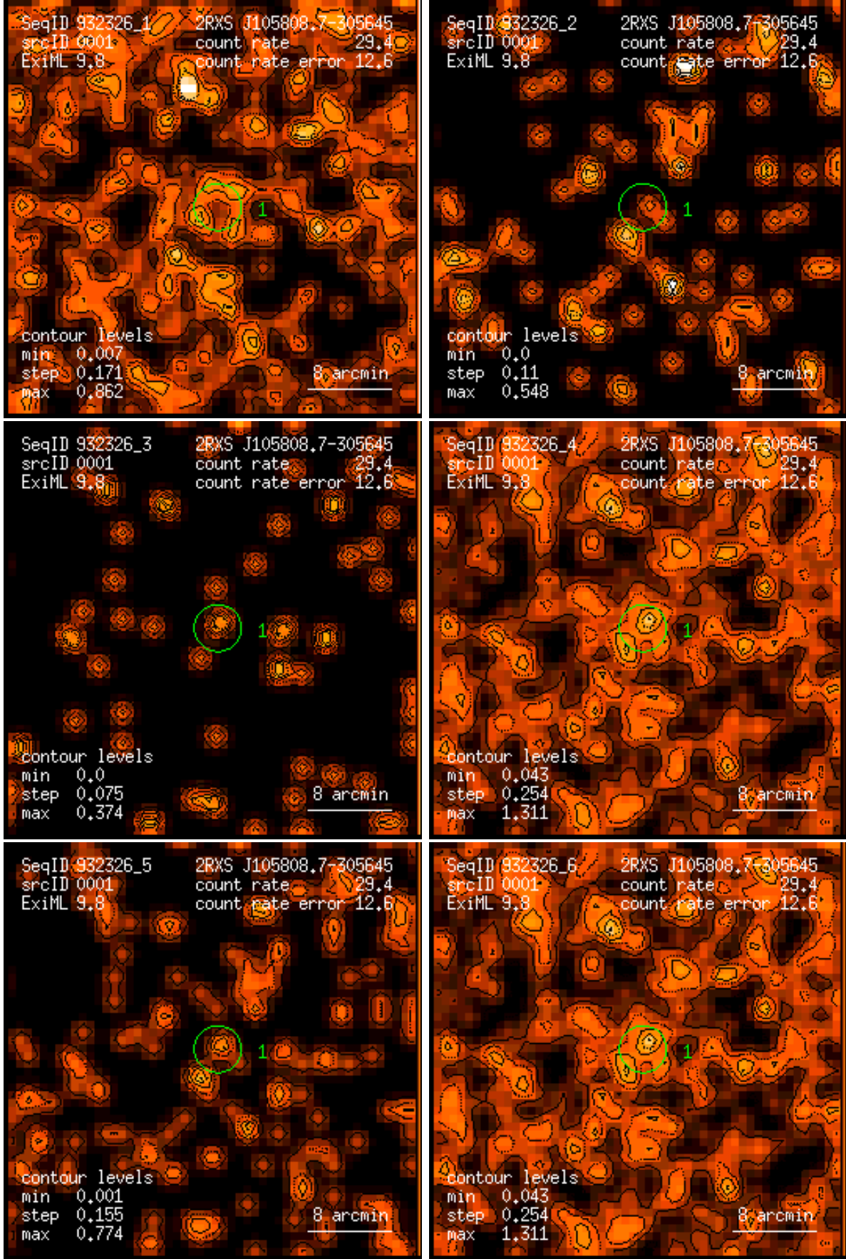
Figure 1: RASS 932326: detection 0001: band rate images, Gaussian filter: (1) PSPC channels 11 – 41, (2) 52 – 90, (3) 91 – 201, (4) 11 – 235, (5) 52 – 201, (6) 11 – 201. Broad band rates in counts/ks. Band rate contour levels in counts/ks/arcmin 2 .
