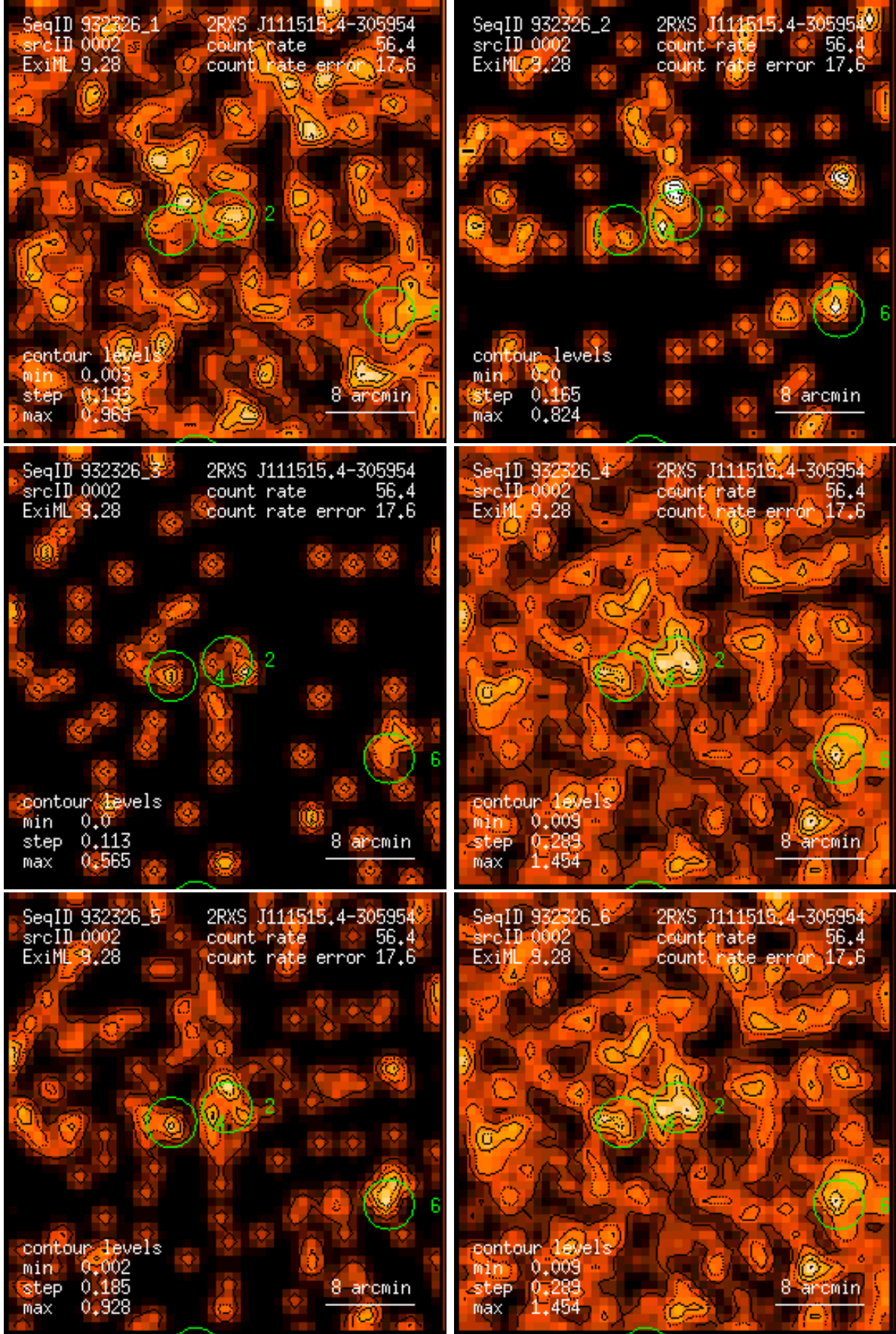
Figure 2: RASS 932326: detection 0002: band rate images, Gaussian filter: (1) PSPC channels 11 – 41, (2) 52 – 90, (3) 91 – 201, (4) 11 – 235, (5) 52 – 201, (6) 11 – 201. Broad band rates in counts/ks. Band rate contour levels in counts/ks/arcmin 2 .
