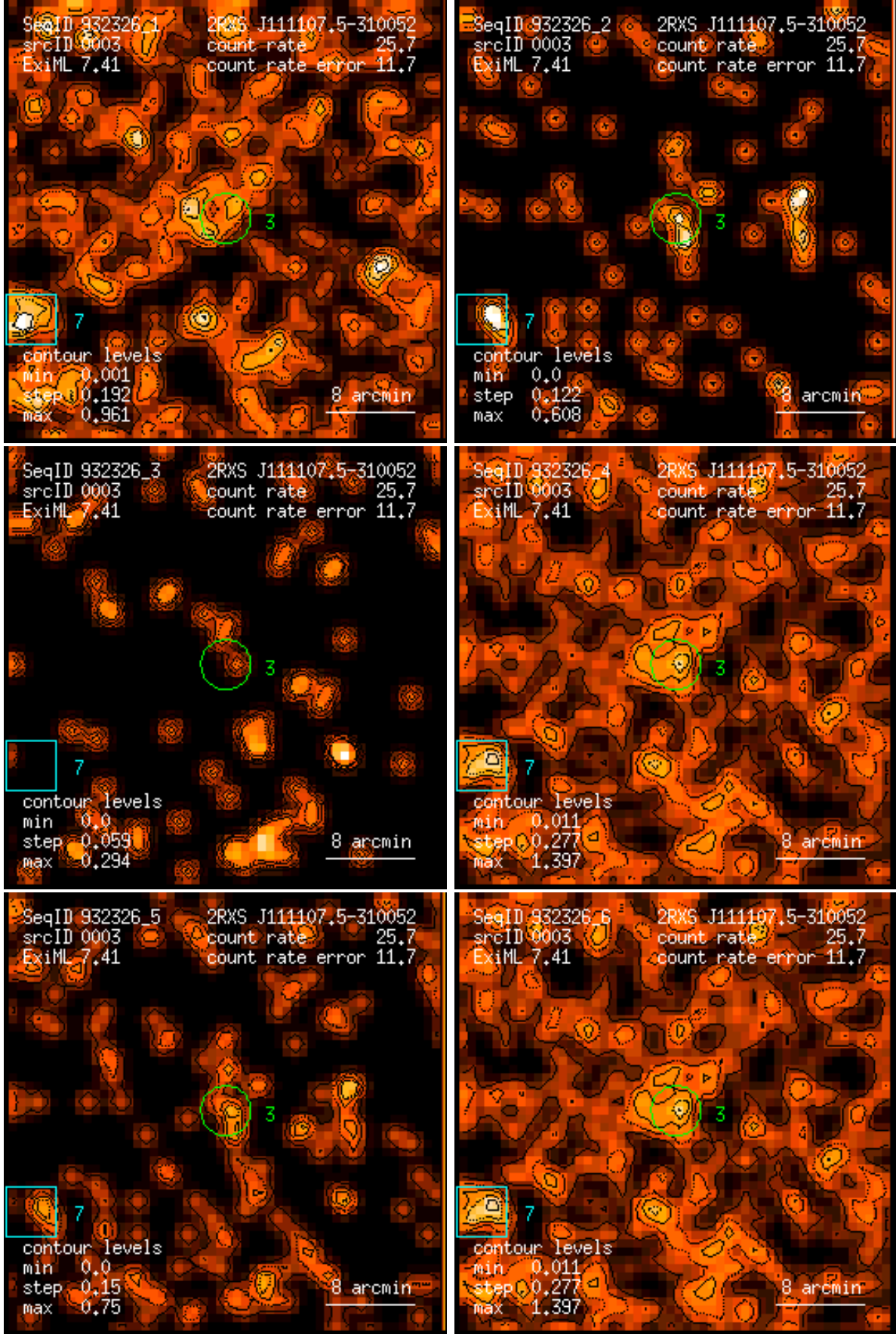
Figure 3: RASS 932326: detection 0003: band rate images, Gaussian filter: (1) PSPC channels 11 – 41, (2) 52 – 90, (3) 91 – 201, (4) 11 – 235, (5) 52 – 201, (6) 11 – 201. Broad band rates in counts/ks. Band rate contour levels in counts/ks/arcmin 2 .
