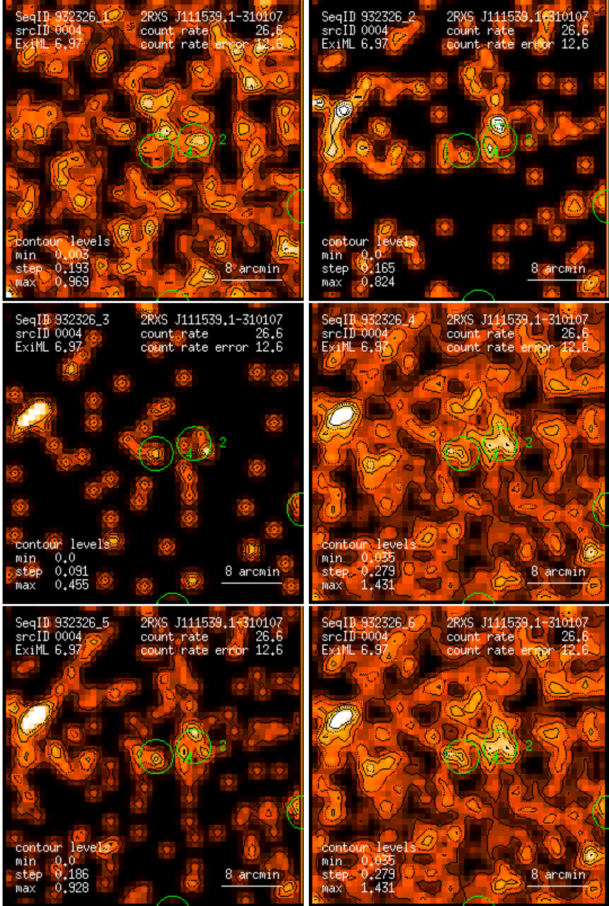
Figure 4: RASS 932326: detection 0004: band rate images, Gaussian filter: (1) PSPC channels 11 – 41, (2) 52 – 90, (3) 91 – 201, (4) 11 – 235, (5) 52 – 201, (6) 11 – 201. Broad band rates in counts/ks. Band rate contour levels in counts/ks/arcmin 2 .
