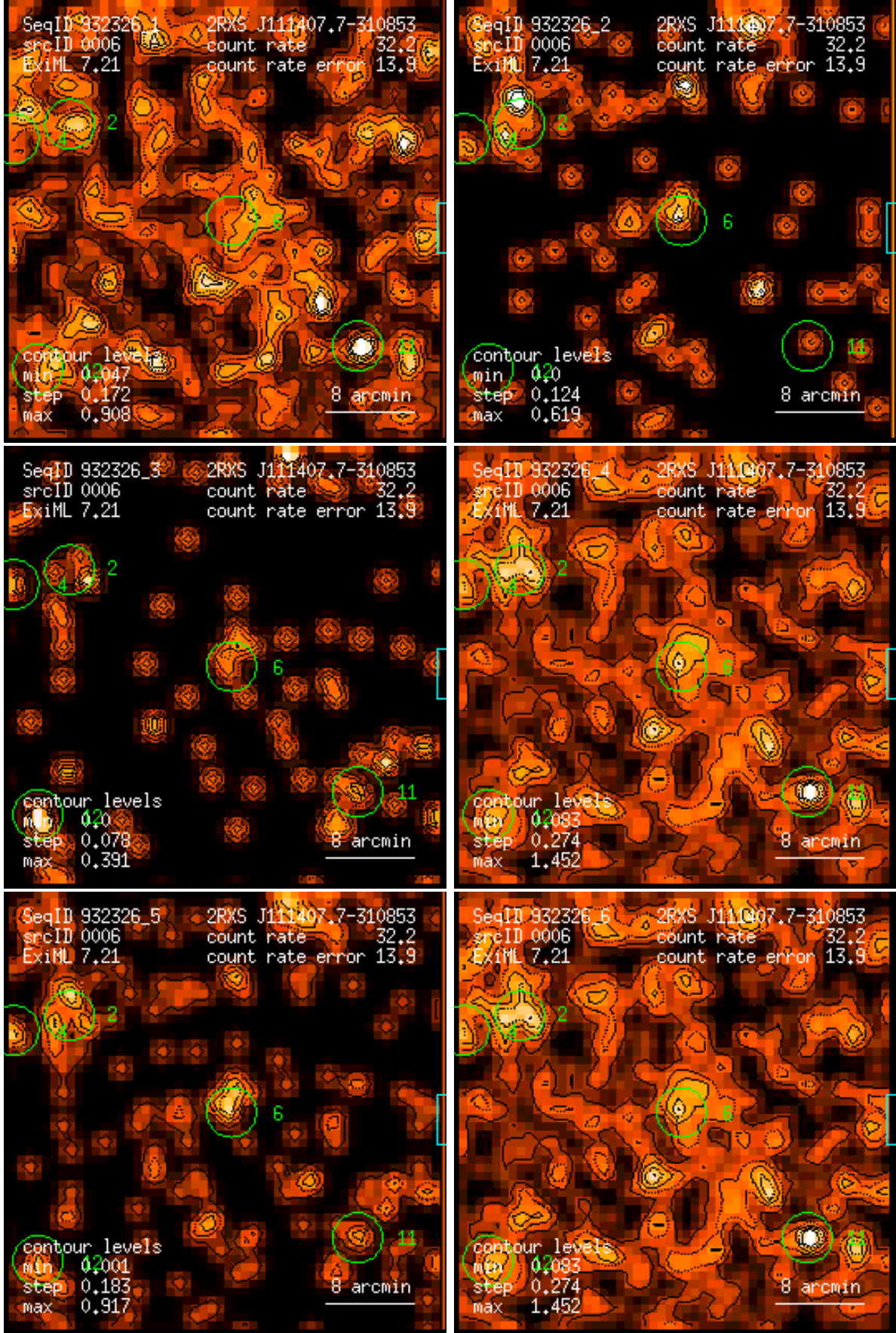
Figure 6: RASS 932326: detection 0006: band rate images, Gaussian filter: (1) PSPC channels 11 – 41, (2) 52 – 90, (3) 91 – 201, (4) 11 – 235, (5) 52 – 201, (6) 11 – 201. Broad band rates in counts/ks. Band rate contour levels in counts/ks/arcmin 2 .
