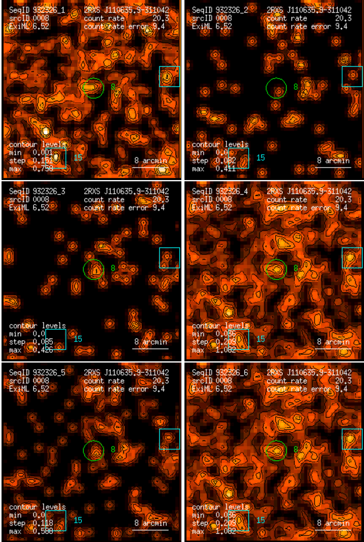
Figure 8: RASS 932326: detection 0008: band rate images, Gaussian filter: (1) PSPC channels 11 – 41, (2) 52 – 90, (3) 91 – 201, (4) 11 – 235, (5) 52 – 201, (6) 11 – 201. Broad band rates in counts/ks. Band rate contour levels in counts/ks/arcmin 2 .
