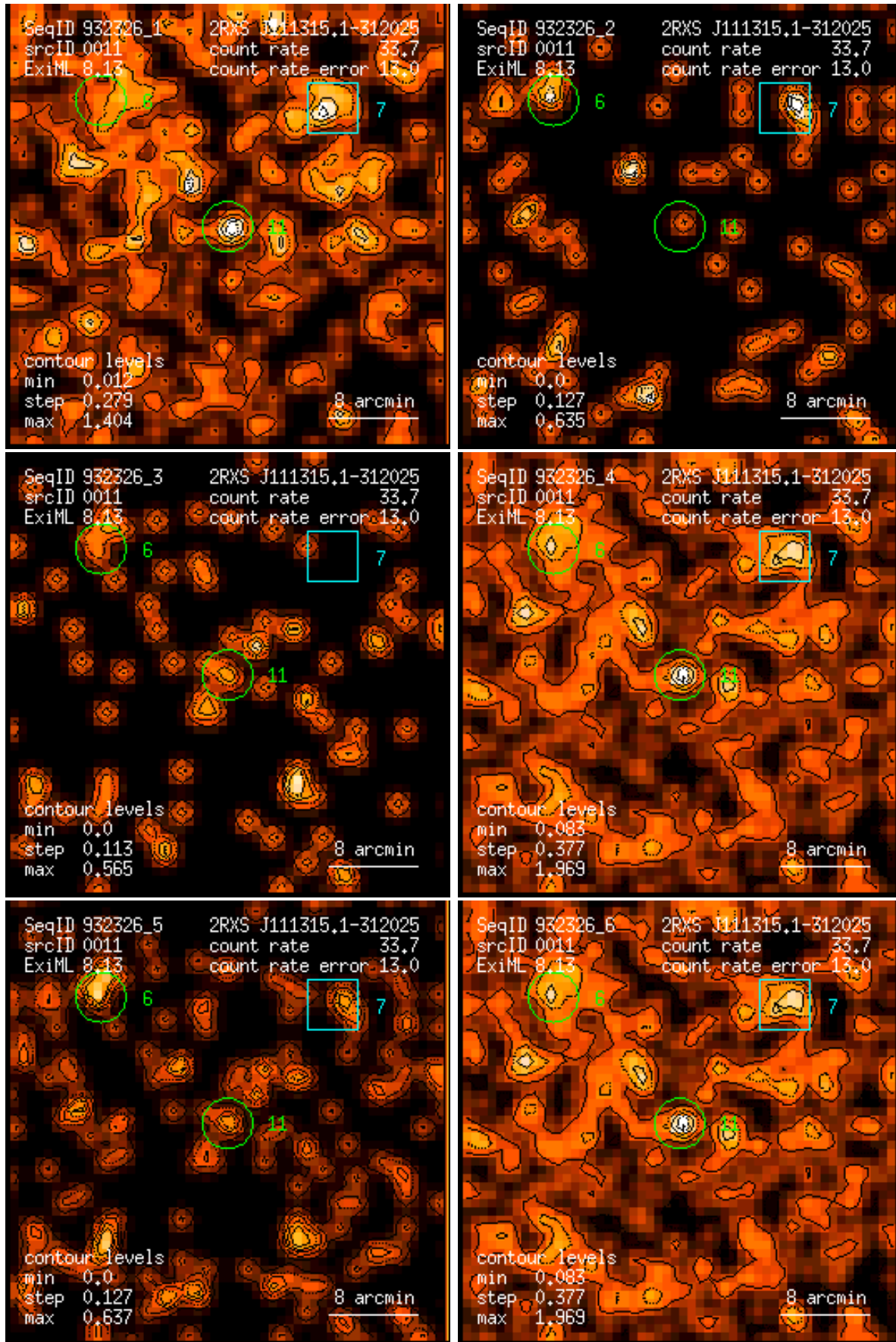
Figure 11: RASS 932326: detection 0011: band rate images, Gaussian filter: (1) PSPC channels 11 – 41, (2) 52 – 90, (3) 91 – 201, (4) 11 – 235, (5) 52 – 201, (6) 11 – 201. Broad band rates in counts/ks. Band rate contour levels in counts/ks/arcmin 2 .
