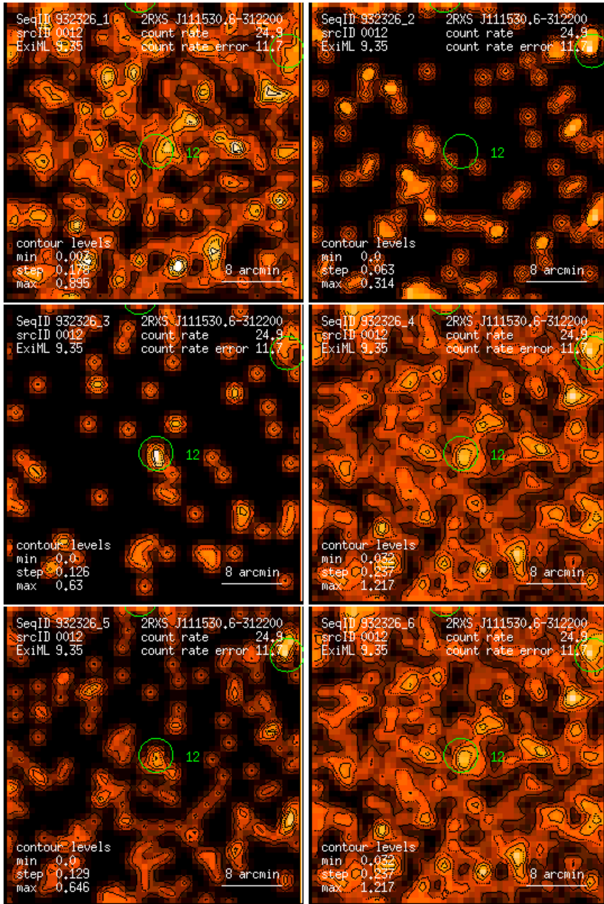
Figure 12: RASS 932326: detection 0012: band rate images, Gaussian filter: (1) PSPC channels 11 – 41, (2) 52 – 90, (3) 91 – 201, (4) 11 – 235, (5) 52 – 201, (6) 11 – 201. Broad band rates in counts/ks. Band rate contour levels in counts/ks/arcmin 2 .
