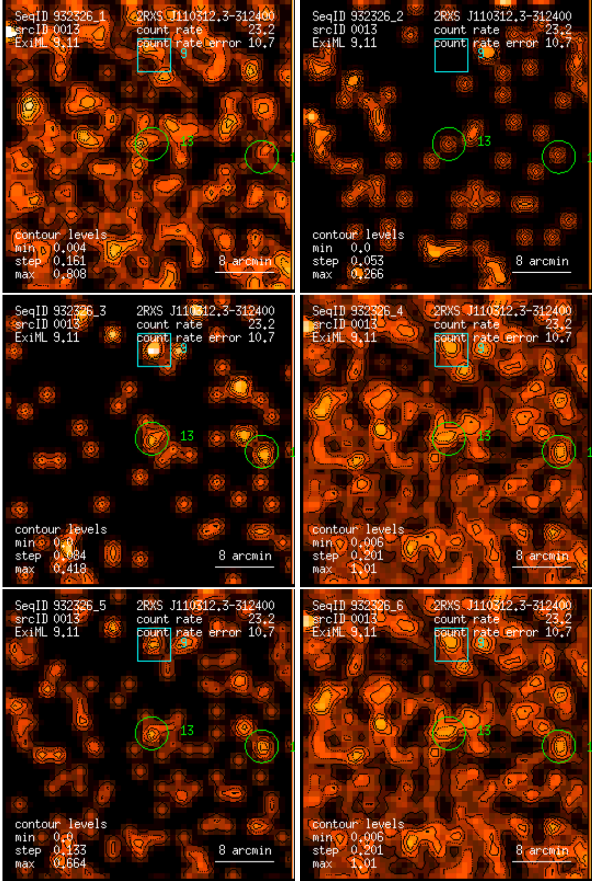
Figure 13: RASS 932326: detection 0013: band rate images, Gaussian filter: (1) PSPC channels 11 – 41, (2) 52 – 90, (3) 91 – 201, (4) 11 – 235, (5) 52 – 201, (6) 11 – 201. Broad band rates in counts/ks. Band rate contour levels in counts/ks/arcmin 2 .
