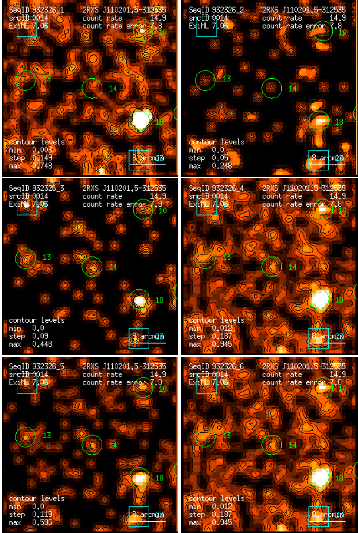
Figure 14: RASS 932326: detection 0014: band rate images, Gaussian filter: (1) PSPC channels 11 – 41, (2) 52 – 90, (3) 91 – 201, (4) 11 – 235, (5) 52 – 201, (6) 11 – 201. Broad band rates in counts/ks. Band rate contour levels in counts/ks/arcmin 2 .
