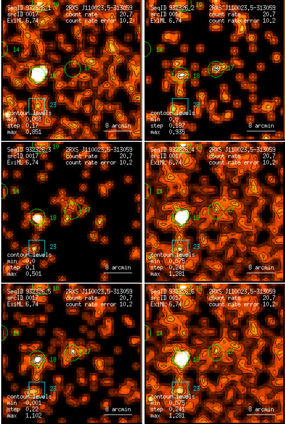
Figure 17: RASS 932326: detection 0017: band rate images, Gaussian filter: (1) PSPC channels 11 – 41, (2) 52 – 90, (3) 91 – 201, (4) 11 – 235, (5) 52 – 201, (6) 11 – 201. Broad band rates in counts/ks. Band rate contour levels in counts/ks/arcmin 2 .
