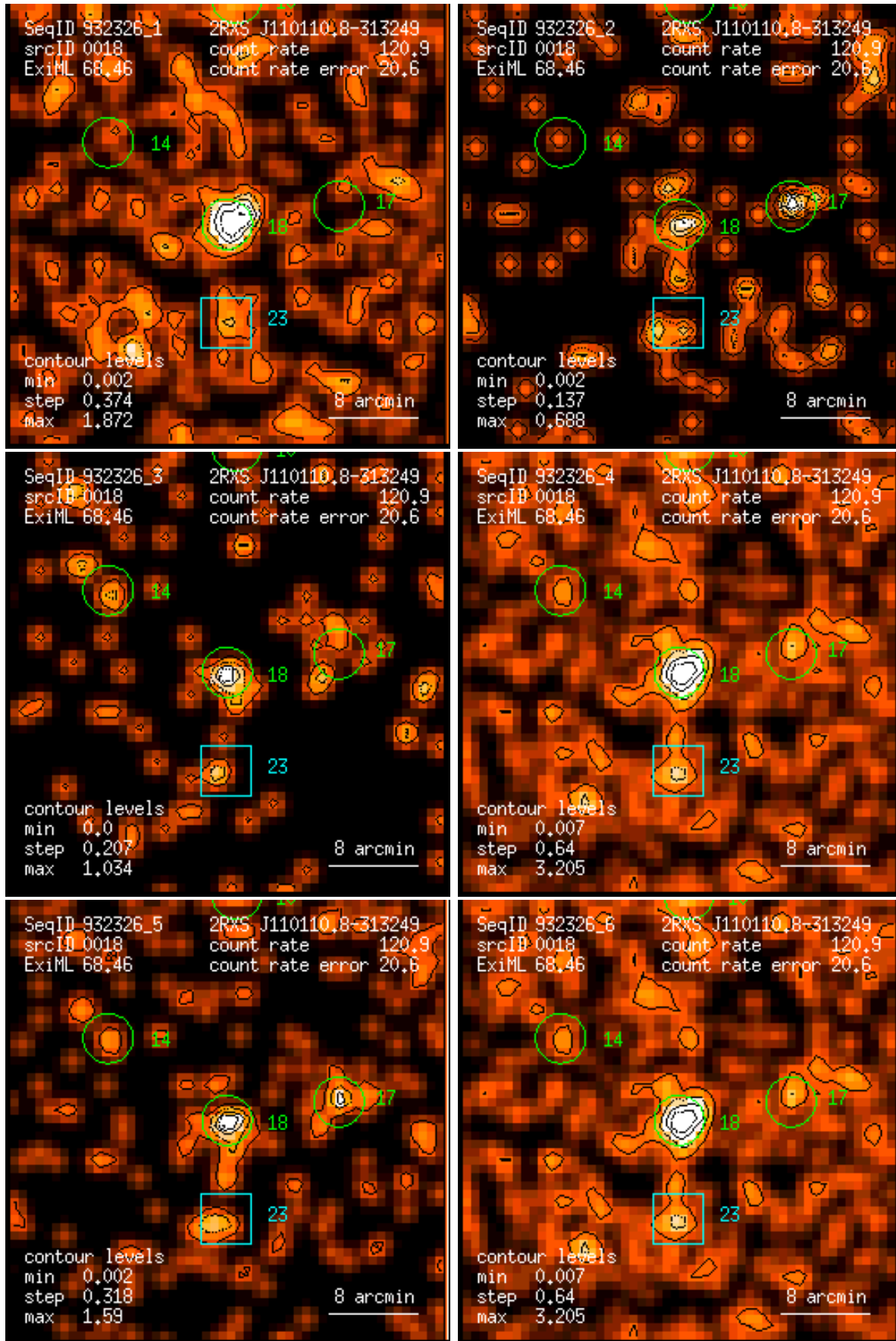
Figure 18: RASS 932326: detection 0018: band rate images, Gaussian filter: (1) PSPC channels 11 – 41, (2) 52 – 90, (3) 91 – 201, (4) 11 – 235, (5) 52 – 201, (6) 11 – 201. Broad band rates in counts/ks. Band rate contour levels in counts/ks/arcmin 2 .
