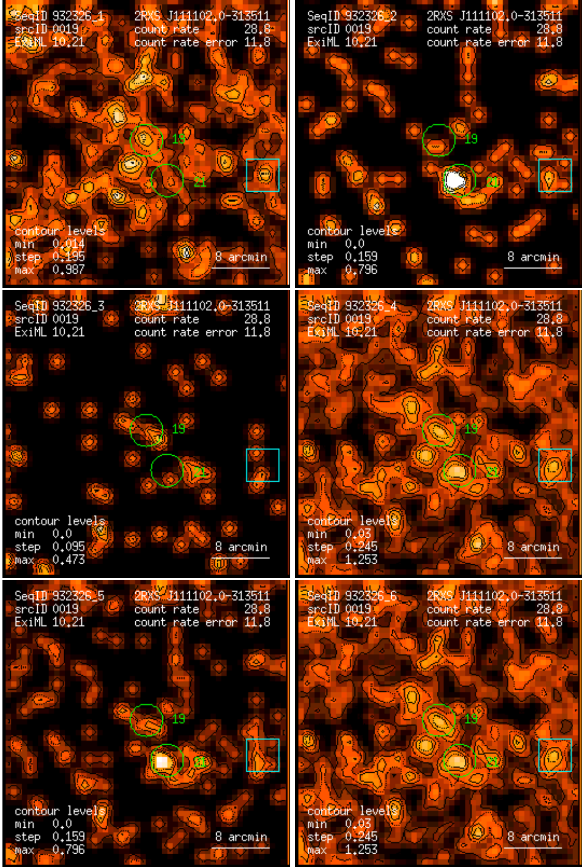
Figure 19: RASS 932326: detection 0019: band rate images, Gaussian filter: (1) PSPC channels 11 – 41, (2) 52 – 90, (3) 91 – 201, (4) 11 – 235, (5) 52 – 201, (6) 11 – 201. Broad band rates in counts/ks. Band rate contour levels in counts/ks/arcmin 2 .
