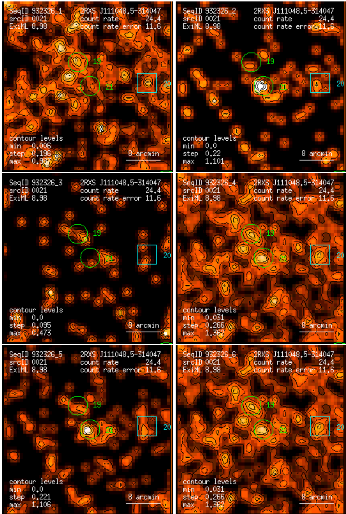
Figure 21: RASS 932326: detection 0021: band rate images, Gaussian filter: (1) PSPC channels 11 – 41, (2) 52 – 90, (3) 91 – 201, (4) 11 – 235, (5) 52 – 201, (6) 11 – 201. Broad band rates in counts/ks. Band rate contour levels in counts/ks/arcmin 2 .
