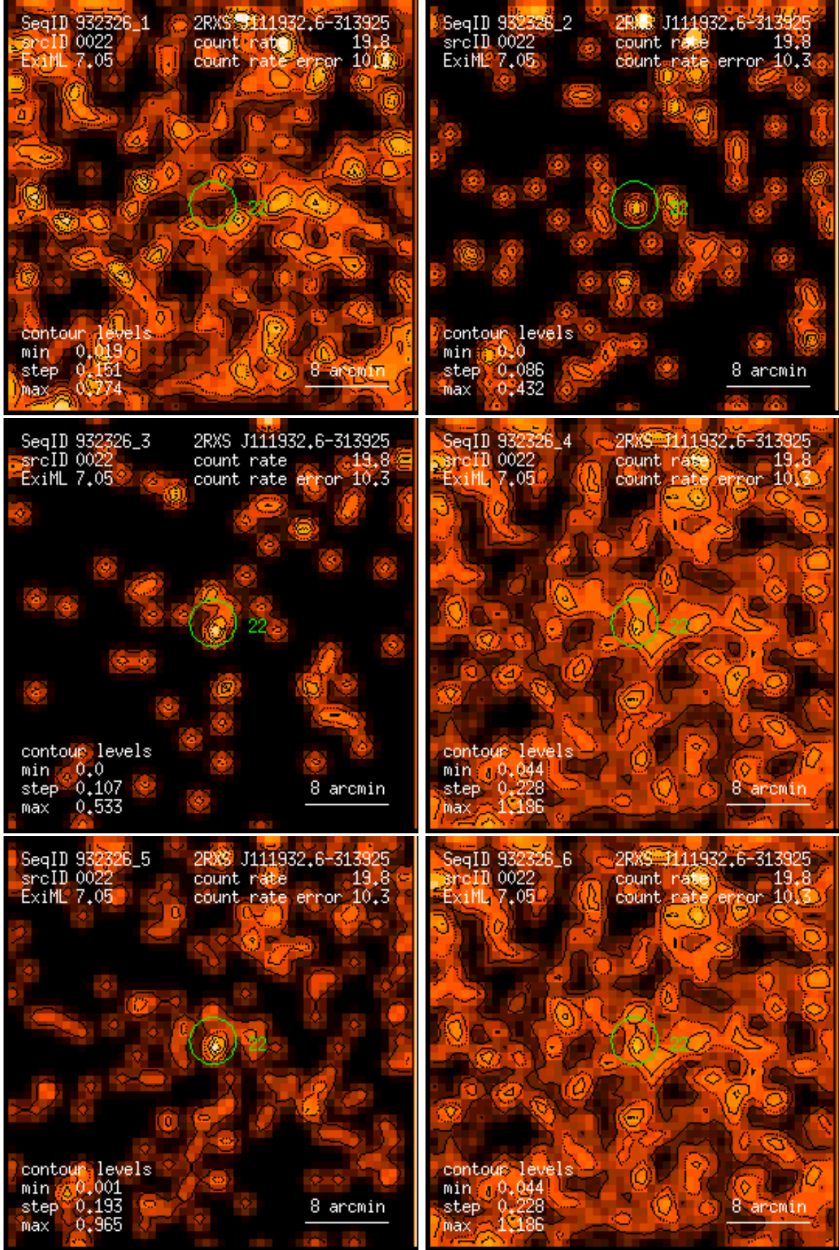
Figure 22: RASS 932326: detection 0022: band rate images, Gaussian filter: (1) PSPC channels 11 – 41, (2) 52 – 90, (3) 91 – 201, (4) 11 – 235, (5) 52 – 201, (6) 11 – 201. Broad band rates in counts/ks. Band rate contour levels in counts/ks/arcmin 2 .
