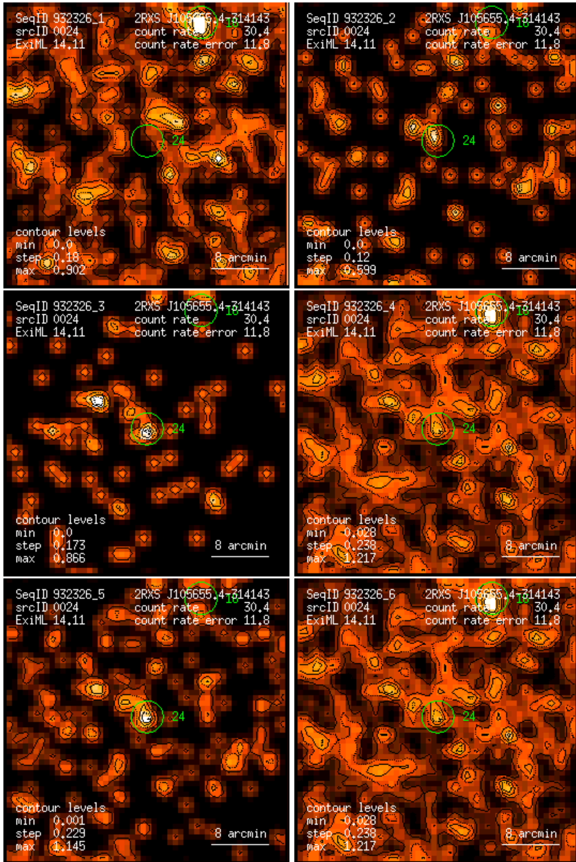
Figure 24: RASS 932326: detection 0024: band rate images, Gaussian filter: (1) PSPC channels 11 – 41, (2) 52 – 90, (3) 91 – 201, (4) 11 – 235, (5) 52 – 201, (6) 11 – 201. Broad band rates in counts/ks. Band rate contour levels in counts/ks/arcmin 2 .
