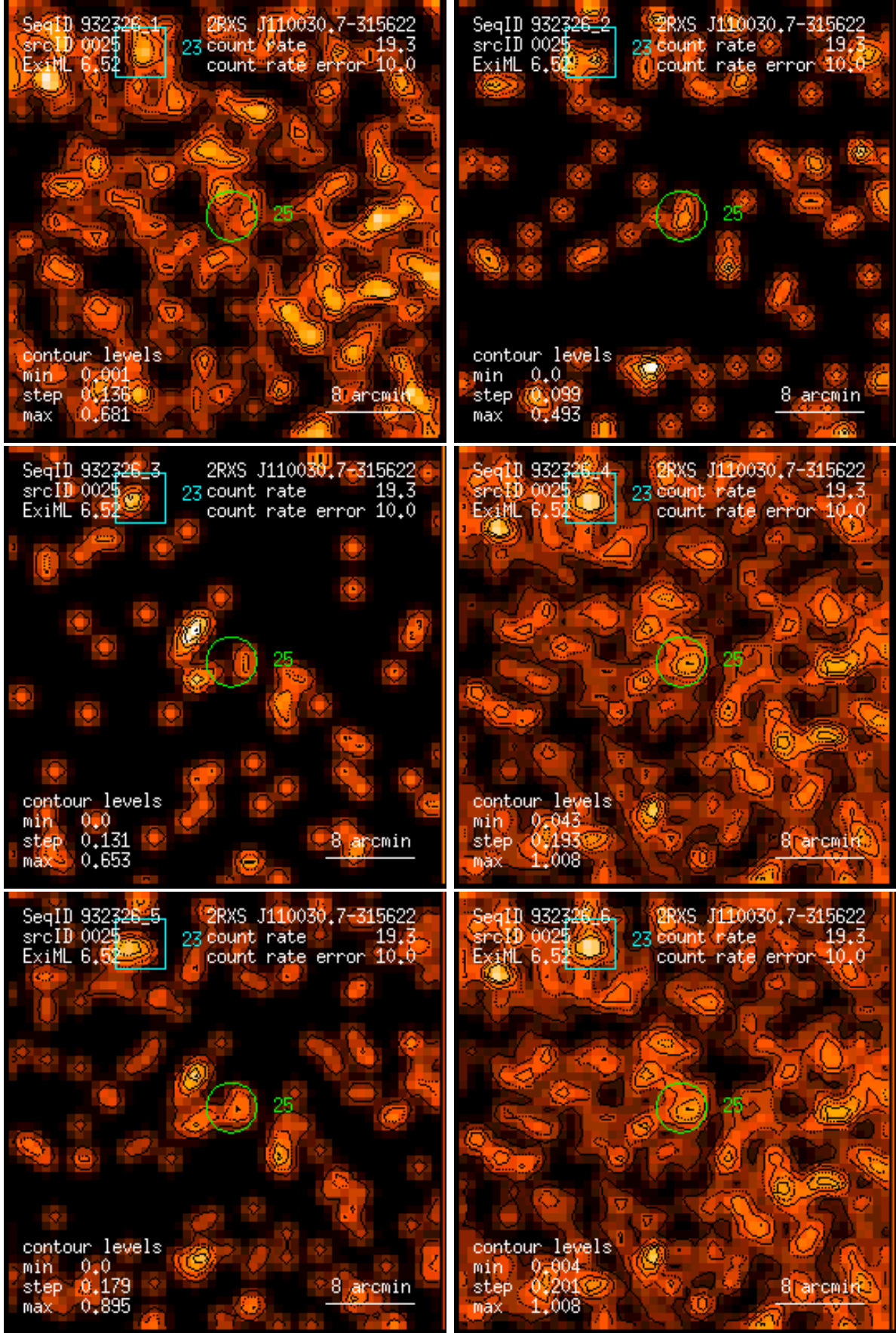
Figure 25: RASS 932326: detection 0025: band rate images, Gaussian filter: (1) PSPC channels 11 – 41, (2) 52 – 90, (3) 91 – 201, (4) 11 – 235, (5) 52 – 201, (6) 11 – 201. Broad band rates in counts/ks. Band rate contour levels in counts/ks/arcmin 2 .
