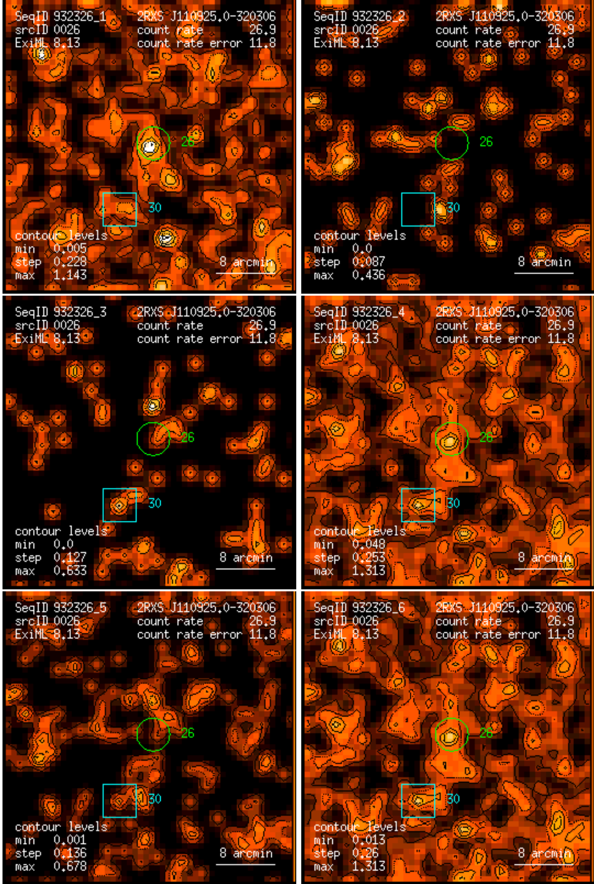
Figure 26: RASS 932326: detection 0026: band rate images, Gaussian filter: (1) PSPC channels 11 – 41, (2) 52 – 90, (3) 91 – 201, (4) 11 – 235, (5) 52 – 201, (6) 11 – 201. Broad band rates in counts/ks. Band rate contour levels in counts/ks/arcmin 2 .
