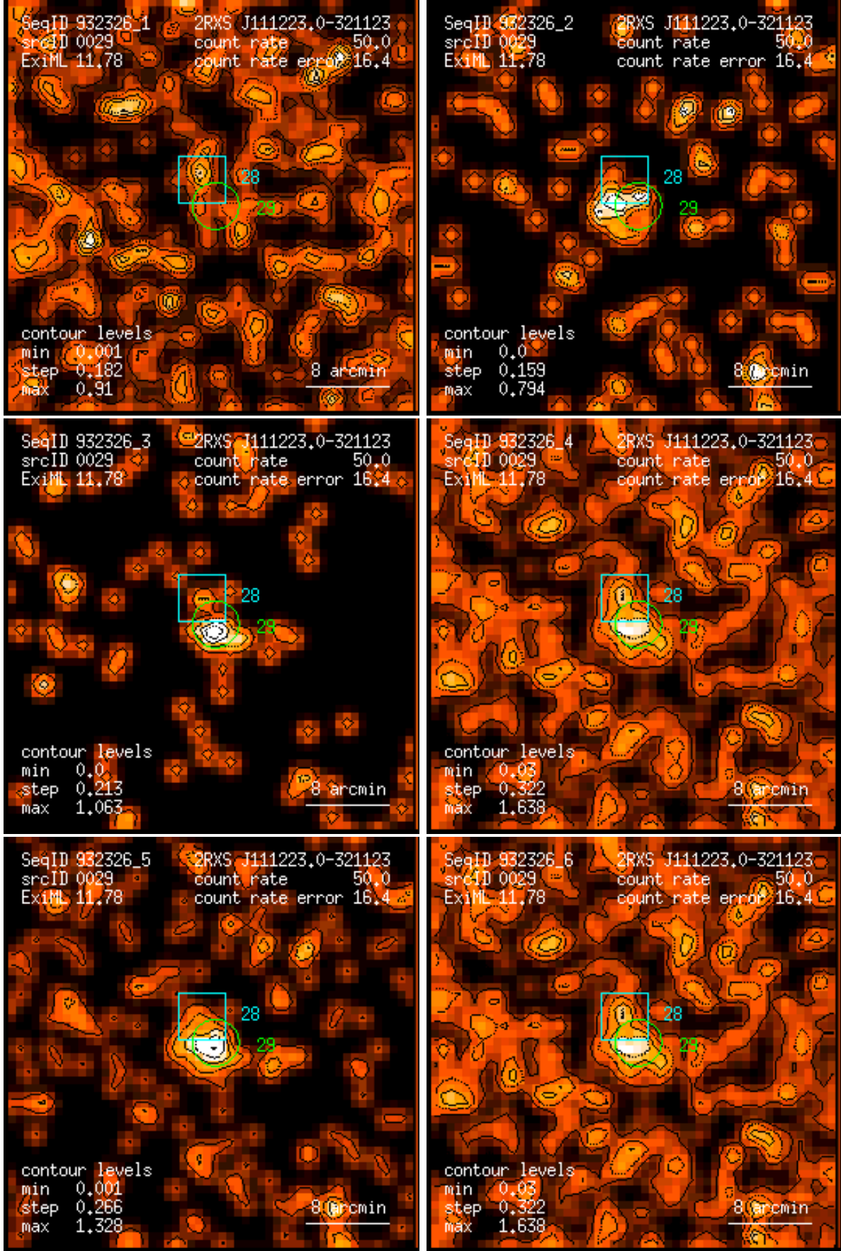
Figure 29: RASS 932326: detection 0029: band rate images, Gaussian filter: (1) PSPC channels 11 – 41, (2) 52 – 90, (3) 91 – 201, (4) 11 – 235, (5) 52 – 201, (6) 11 – 201. Broad band rates in counts/ks. Band rate contour levels in counts/ks/arcmin 2 .
