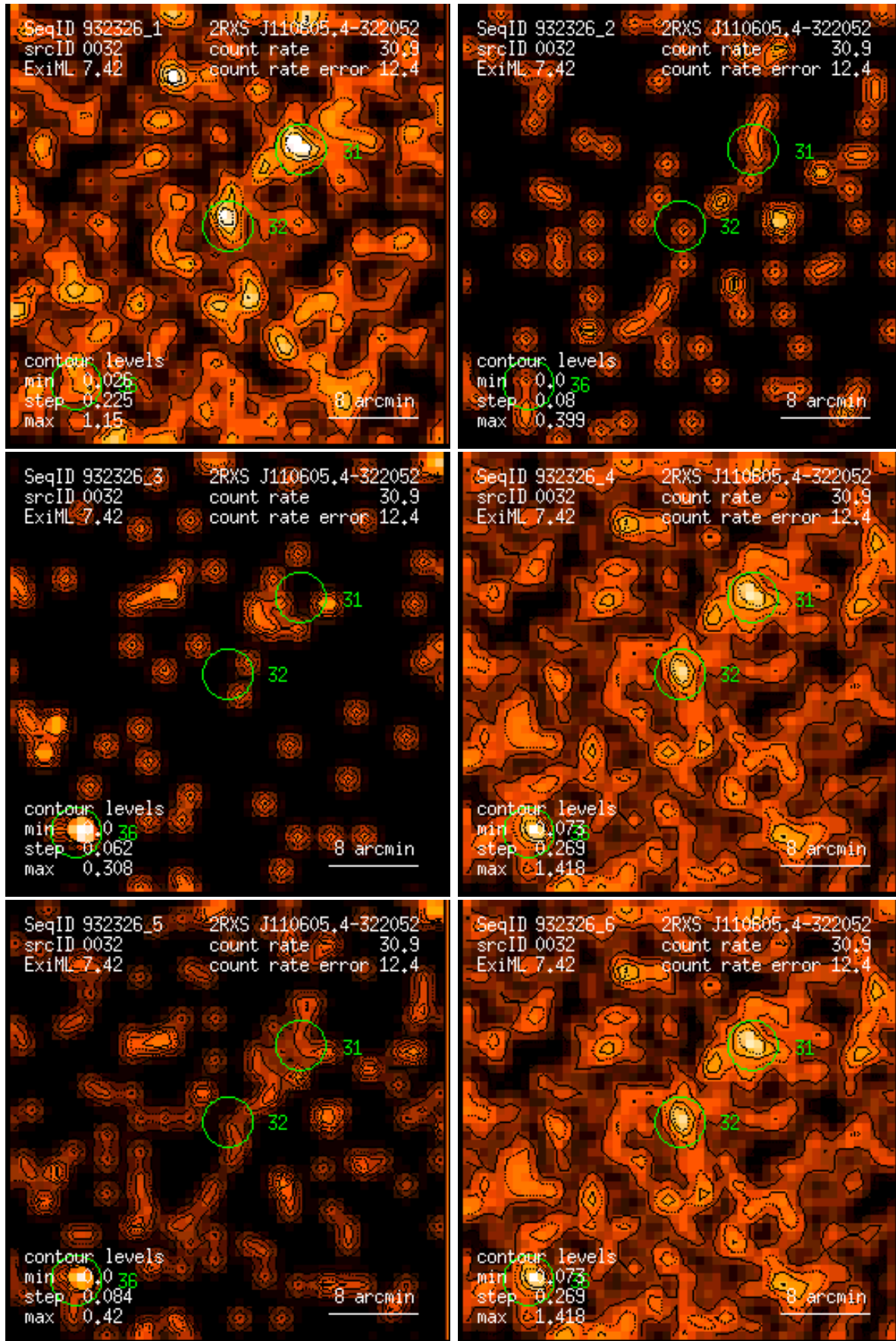
Figure 32: RASS 932326: detection 0032: band rate images, Gaussian filter: (1) PSPC channels 11 – 41, (2) 52 – 90, (3) 91 – 201, (4) 11 – 235, (5) 52 – 201, (6) 11 – 201. Broad band rates in counts/ks. Band rate contour levels in counts/ks/arcmin 2 .
