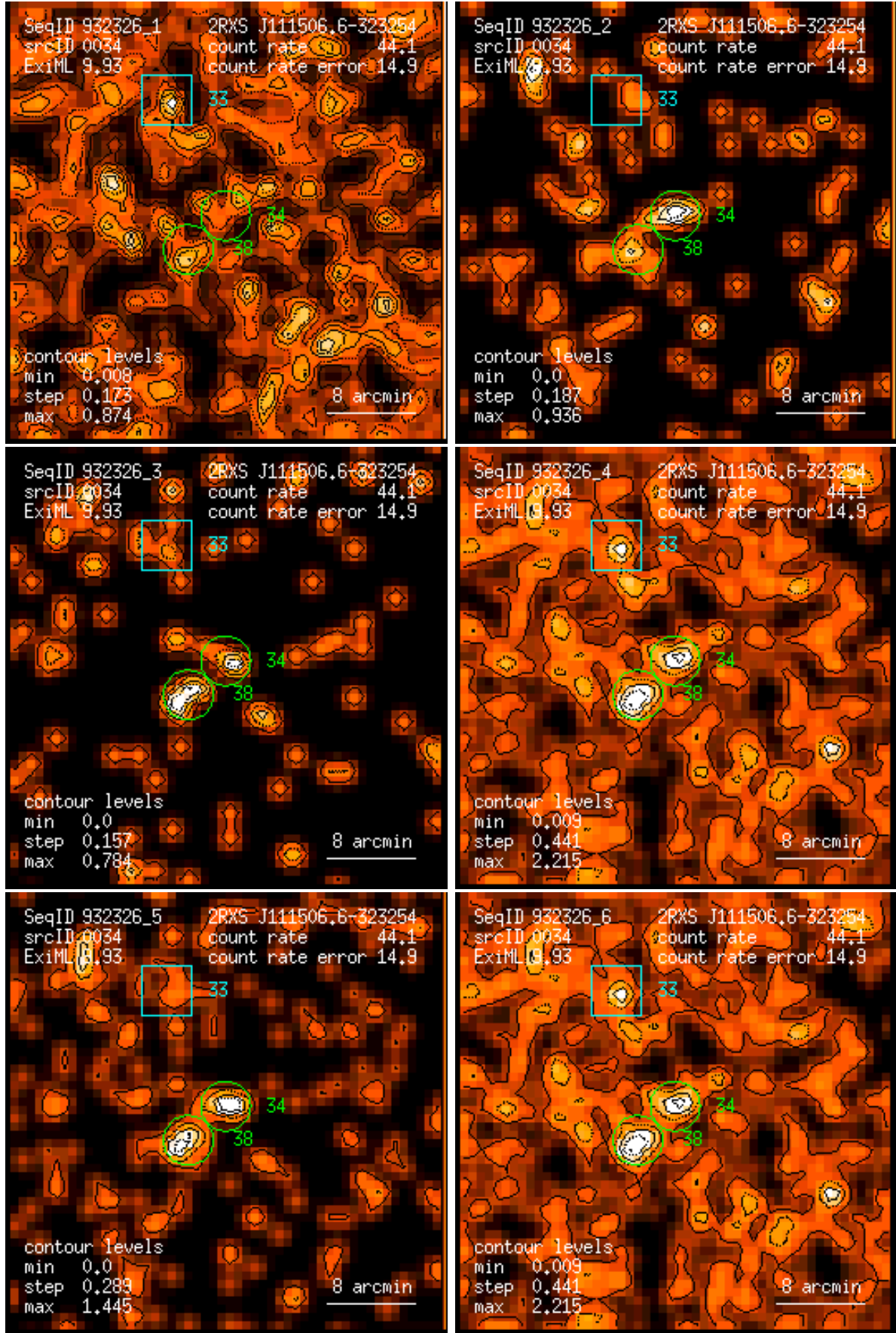
Figure 34: RASS 932326: detection 0034: band rate images, Gaussian filter: (1) PSPC channels 11 – 41, (2) 52 – 90, (3) 91 – 201, (4) 11 – 235, (5) 52 – 201, (6) 11 – 201. Broad band rates in counts/ks. Band rate contour levels in counts/ks/arcmin 2 .
