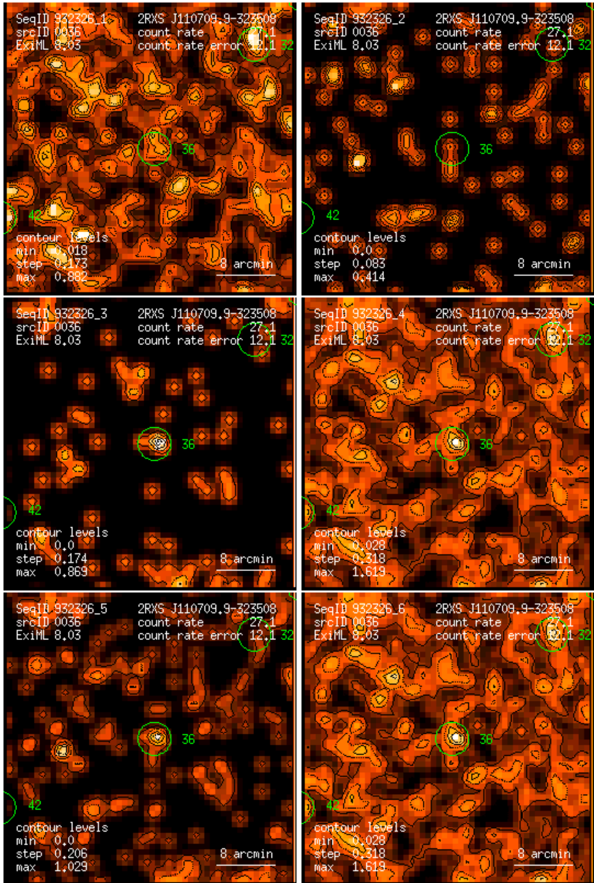
Figure 36: RASS 932326: detection 0036: band rate images, Gaussian filter: (1) PSPC channels 11 – 41, (2) 52 – 90, (3) 91 – 201, (4) 11 – 235, (5) 52 – 201, (6) 11 – 201. Broad band rates in counts/ks. Band rate contour levels in counts/ks/arcmin 2 .
